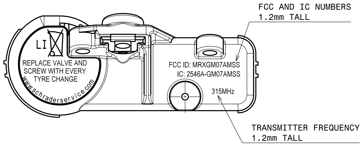
GM07 ENCLOSURE TOP VIEW
