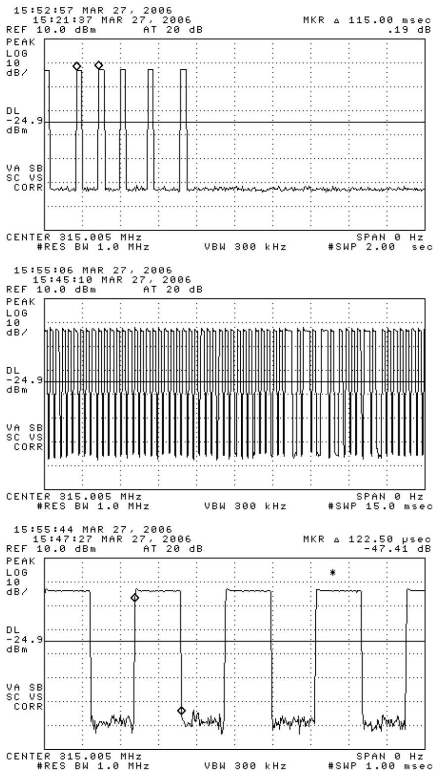
Figure 6.1. Transmissions modulation characteristics: (top) complete transmission, (center) expanded transmission, (bottom) expanded word.
