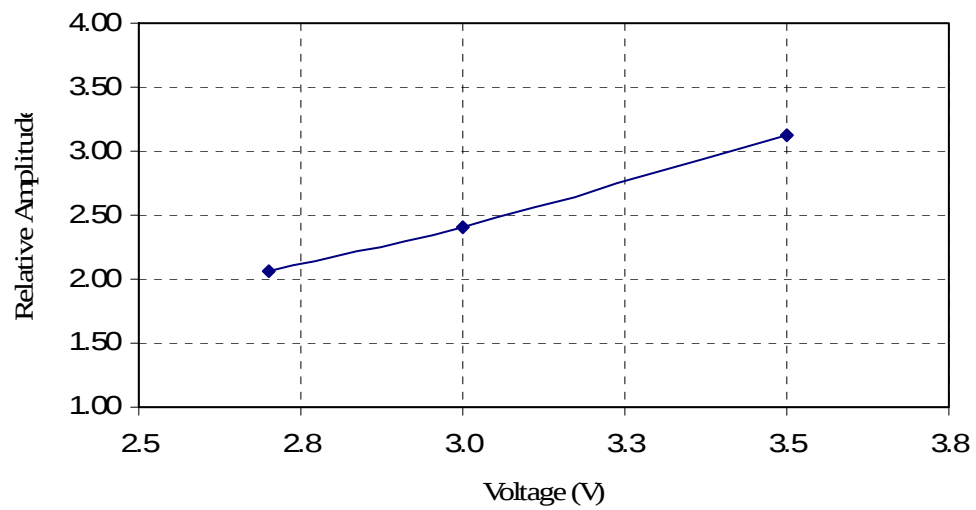
Figure 6.4. Relative emission at 315.0 MHz vs. supply voltage (pulsed emission).
