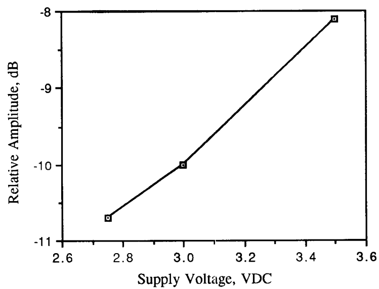
Figure 6.4. Relative emission at 434 MHz vs. supply voltage. (pulsed emission)
