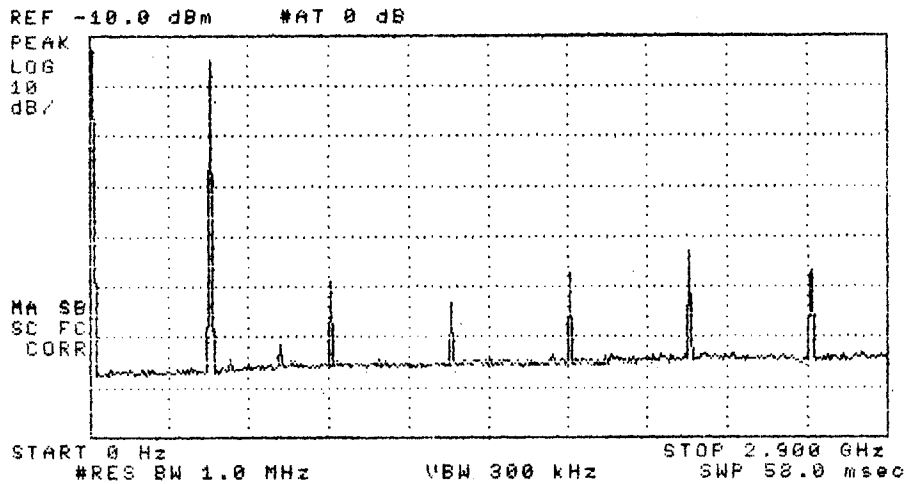
Figure 6.2. Emission spectrum of the DUT in free space (pulsed emission). The amplitudes are only indicative (not calibrated).
