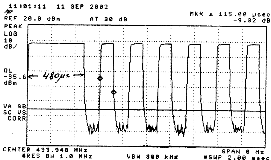
Figure 6.1. Transmissions modulation characteristics: (top) transmission repetition, (center) transmission pulses, (bottom) pulse widths.
