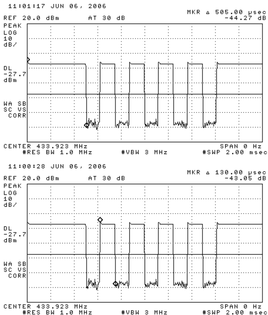
Figure 6.1(b). Transmissions modulation characteristics (cont.).
