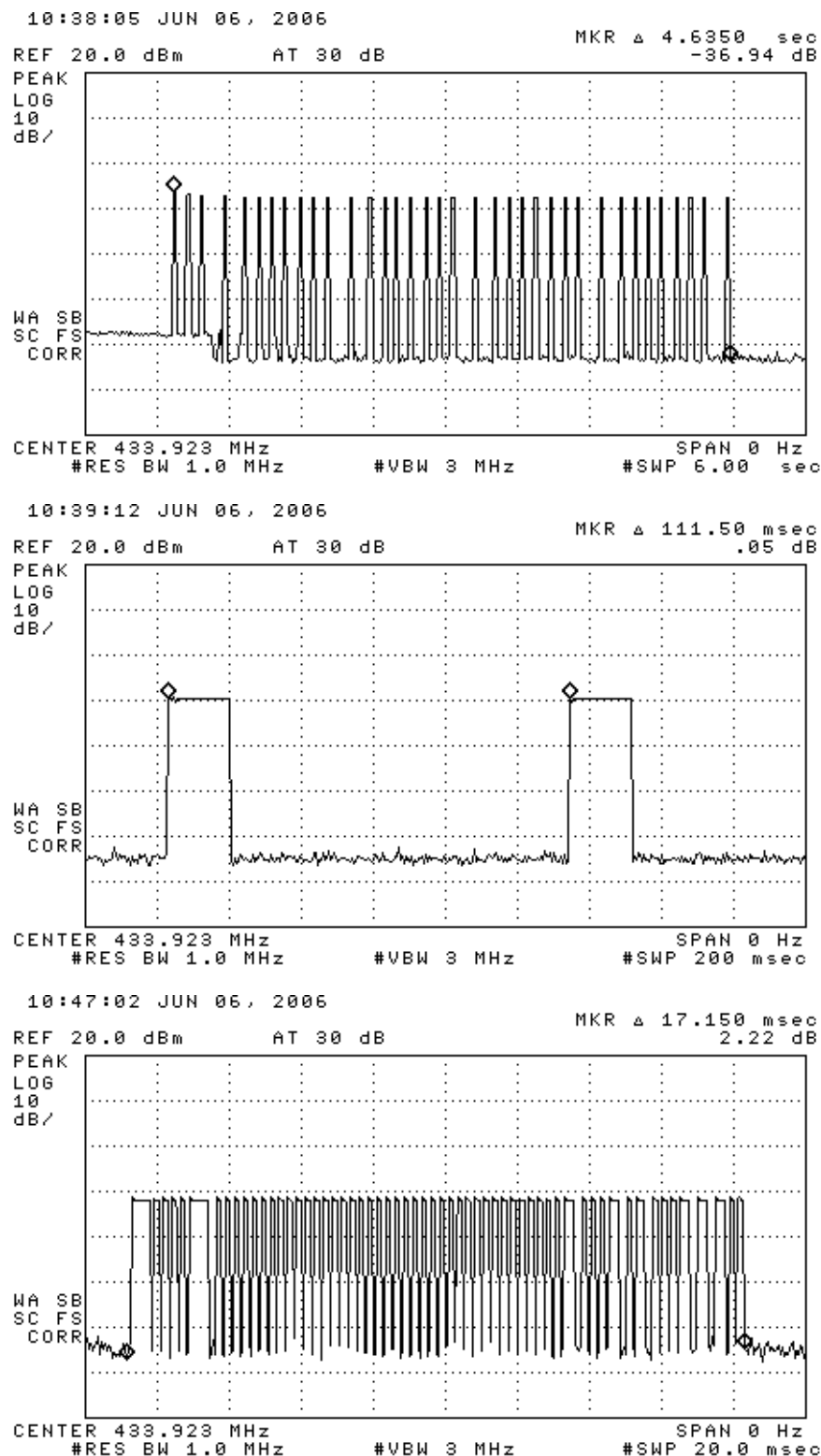
Figure 6.1(a). Transmissions modulation characteristics: (top) complete transmission (LF actuated), (center) expanded period, (bottom) expanded word.
