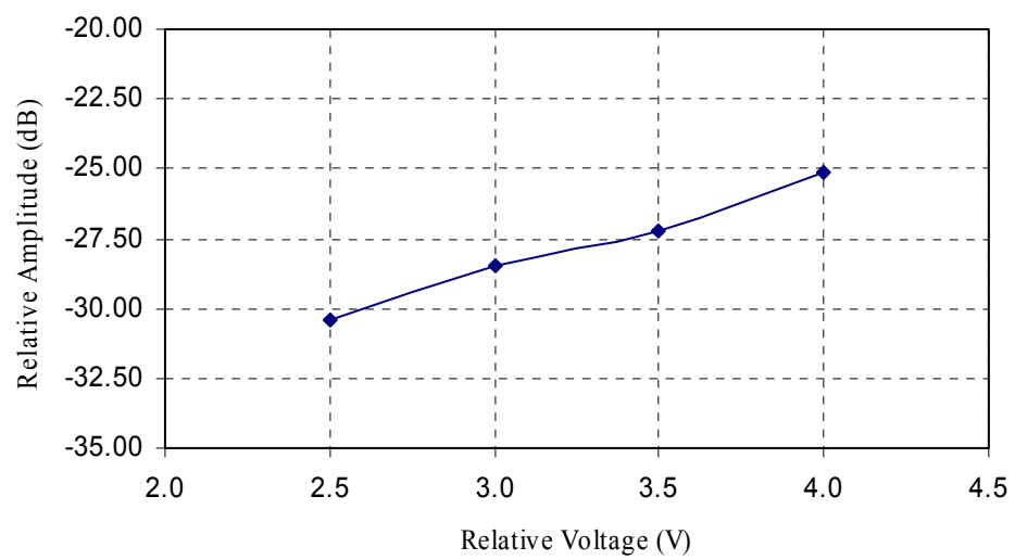
Figure 6.4. Relative emission at 315.0 MHz vs. supply voltage (CW emission).
