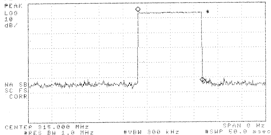
Figure 6.1. Transmissions modulation characteristics: (top) transmission repetition, (center) transmission pulses, (bottom) pulse width.
