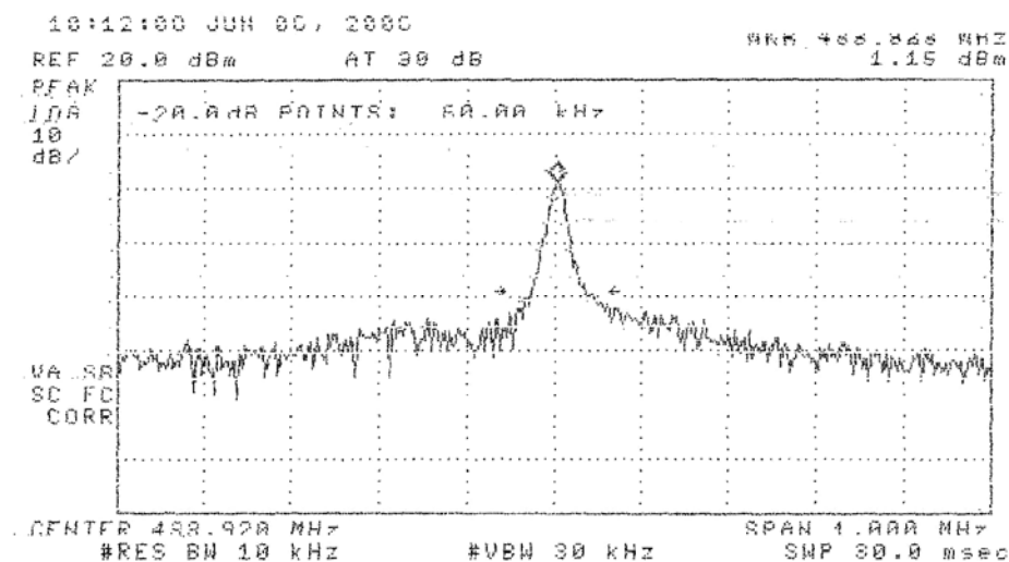
Figure 6.3. Measured bandwidth of the DUT (pulsed emission).
