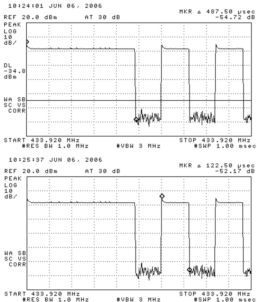
Figure 6.1. Transmissions modulation characteristics (cont.).
