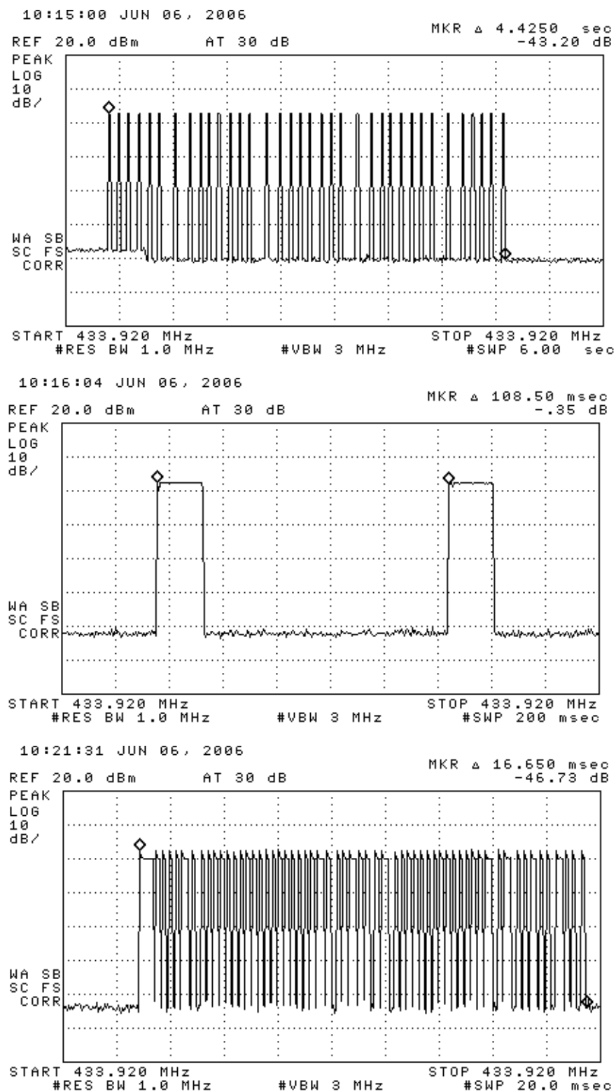
Figure 6.1. Transmissions modulation characteristics: (top) complete transmission, (center) expanded period, (bottom) expanded word.
