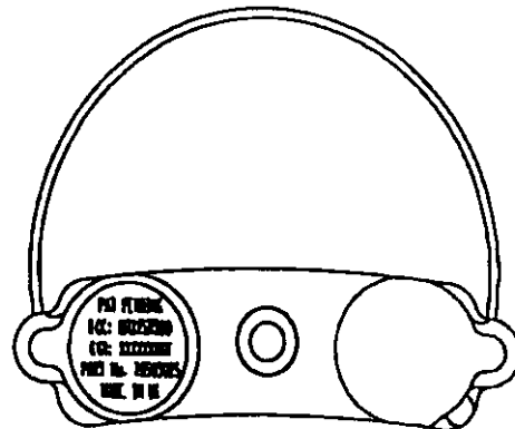
DIAGRAM SHOWING POSITION OF LABEL ON FRONT (UNPOTTED) FACE. (VALVE OMMITED FOR CLARITY).
