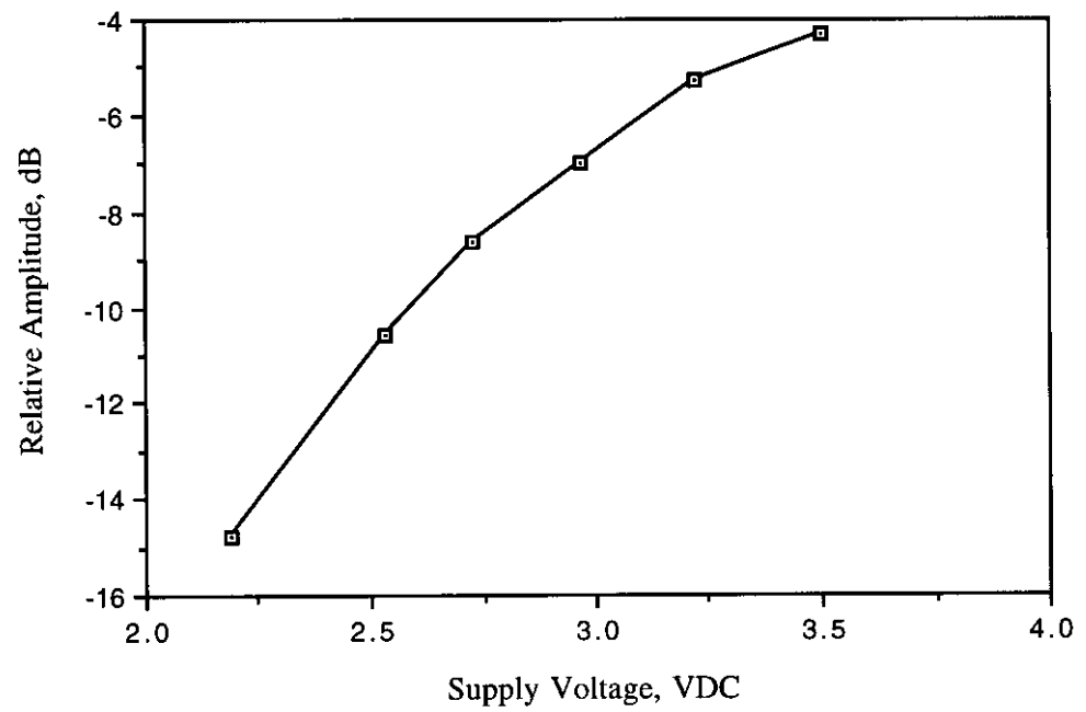
Figure 6.4. Relative emission at 315.0 MHz vs. supply voltage. (CW emission)
