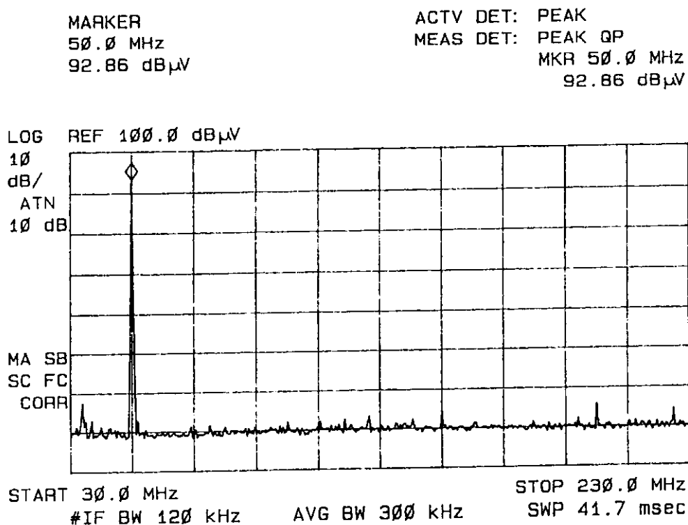
Figure 2 Radiated Emissions @ 1 Meter in Screen Room
