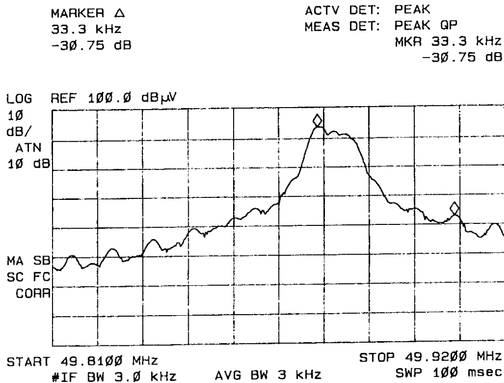
Figure 1 Band Edges
