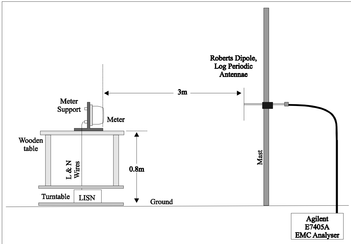
Figure 1: Test Fixture Diagram
