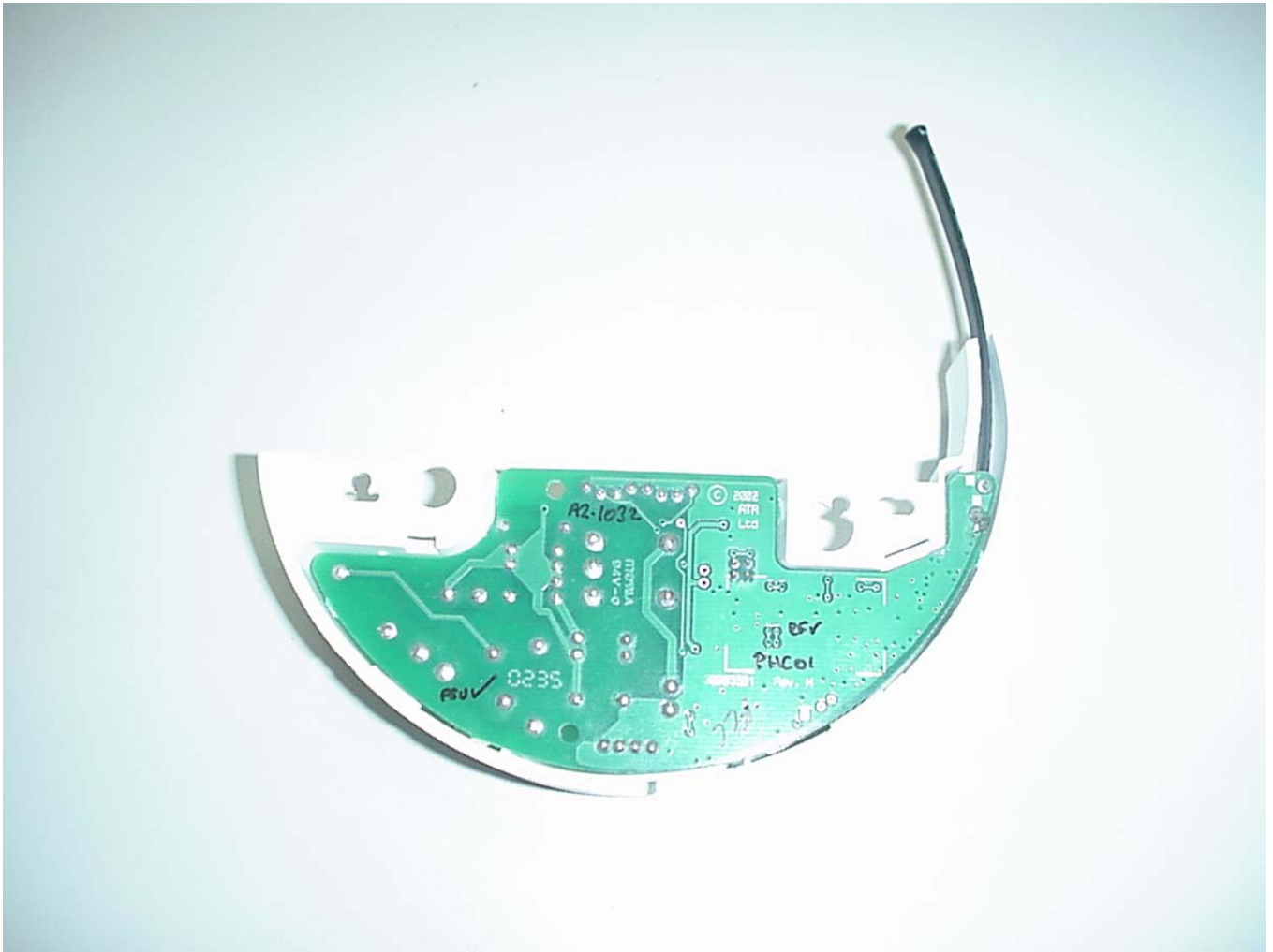
Figure 2 RAMAR EM915 V1.0 Bottom View
