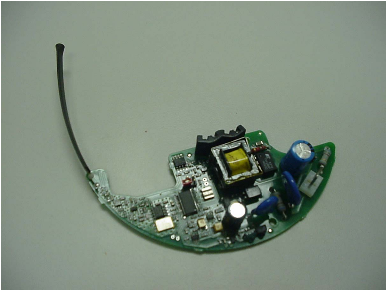
Figure 1 Ramar EM915 V1.0 Top View
