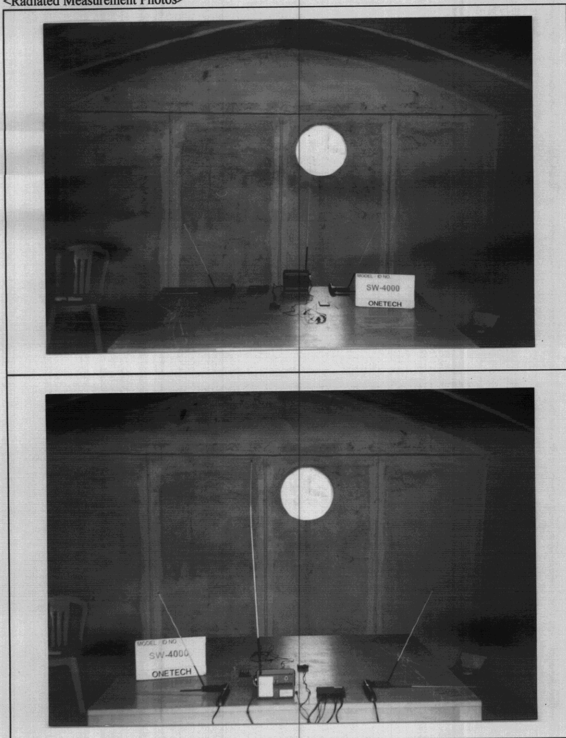
<Radiated Measurement Photos>
