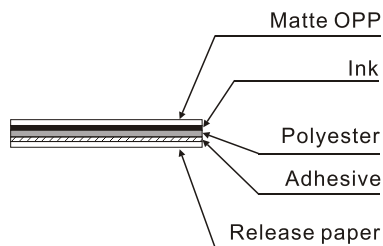
Material Composition Drawing
