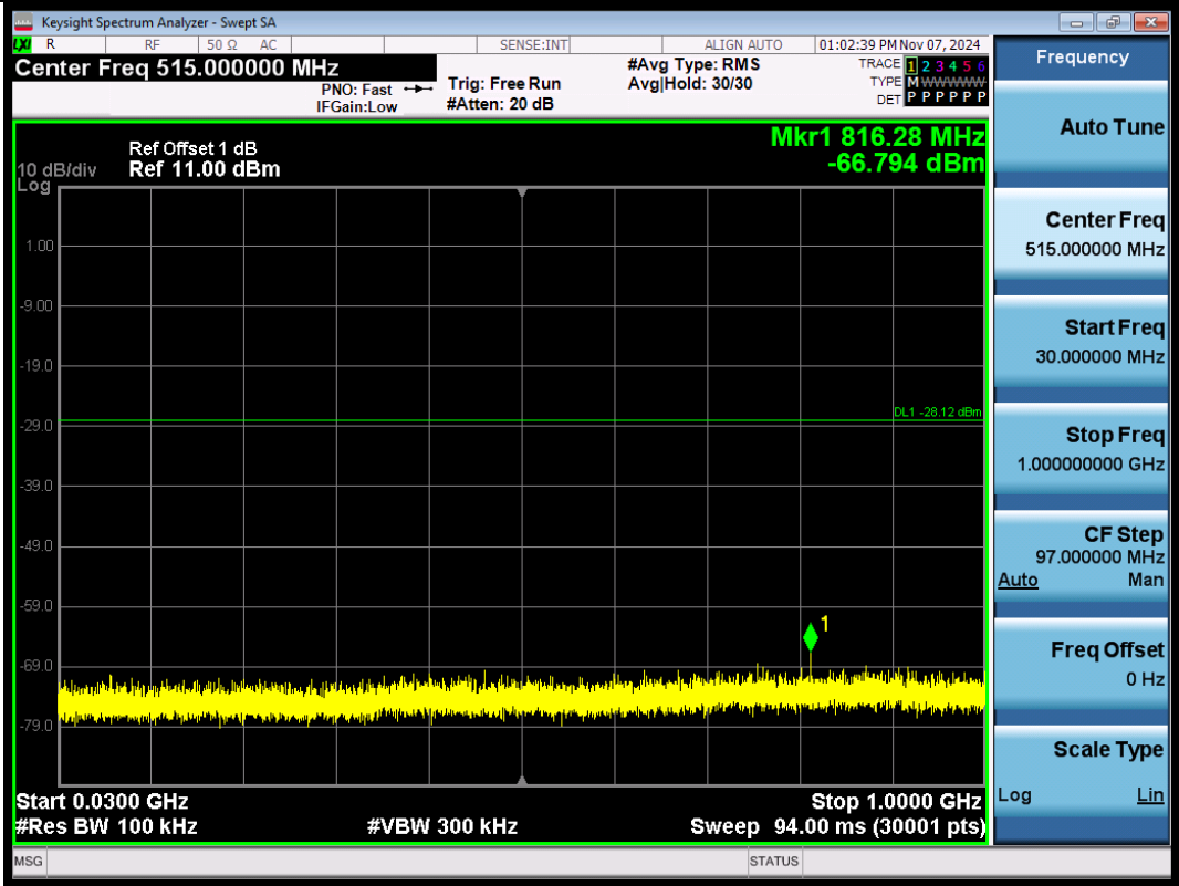
11G-2412-30~1000-PASS
