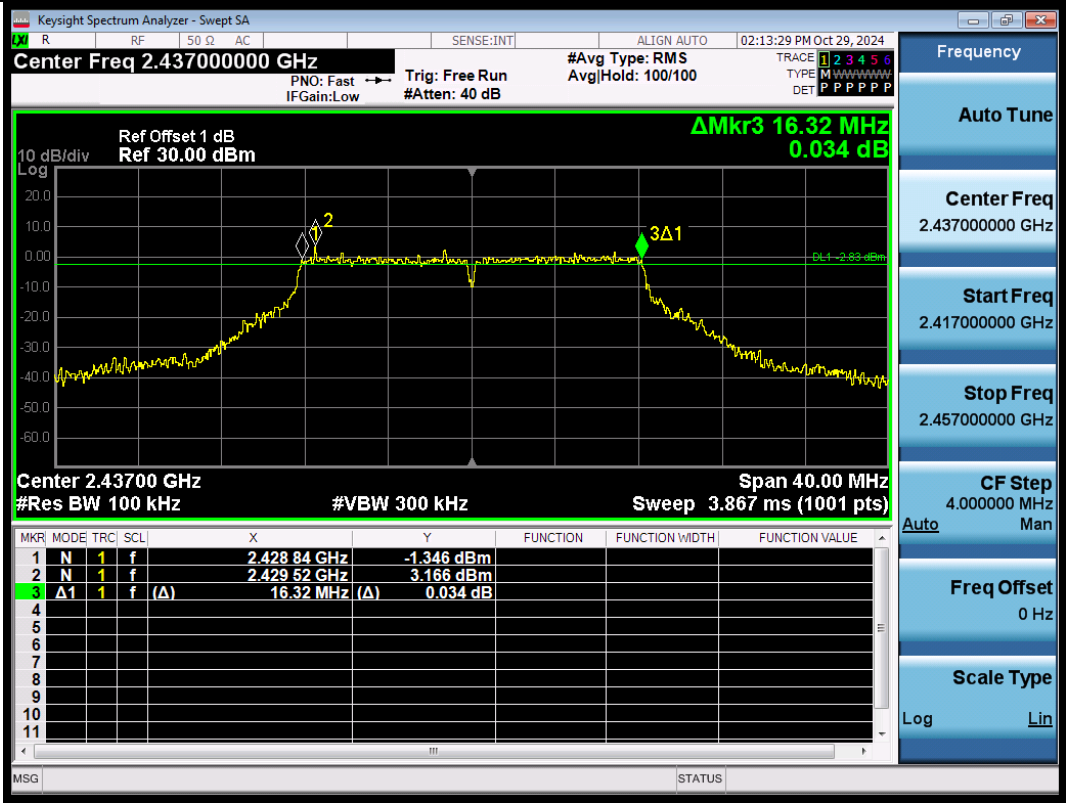
11G-2437-PASS
