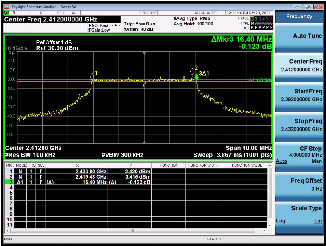
11G-2412-PASS
