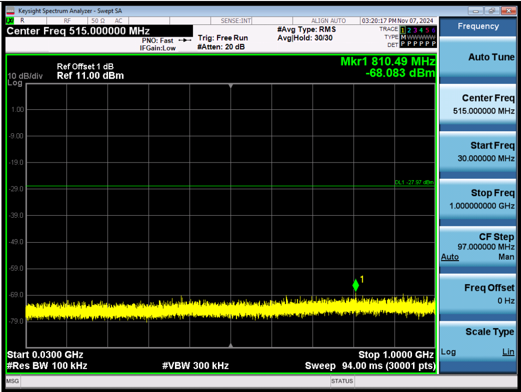
11AX20-2412-30~1000-PASS
