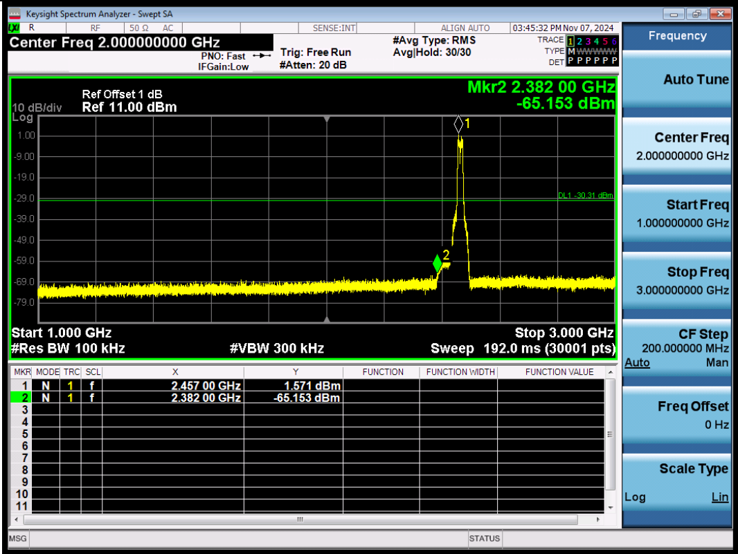
11AX20-2462-1000~3000-PASS
