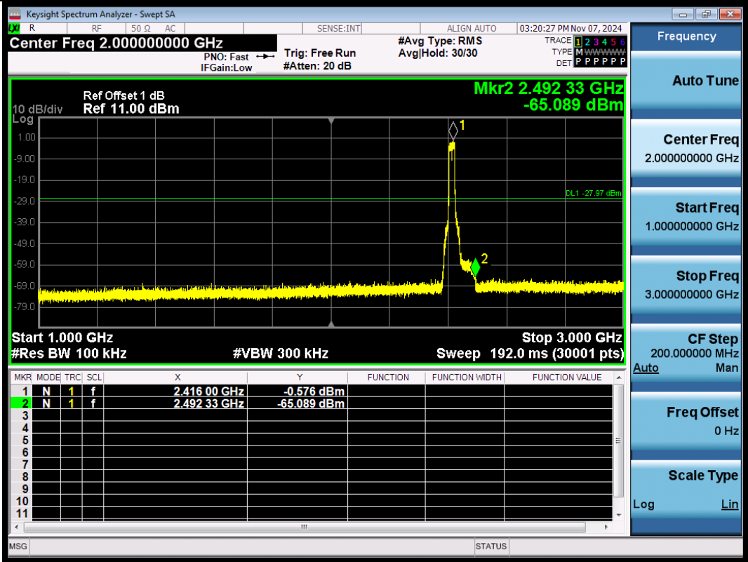
11AX20-2412-1000~3000-PASS
