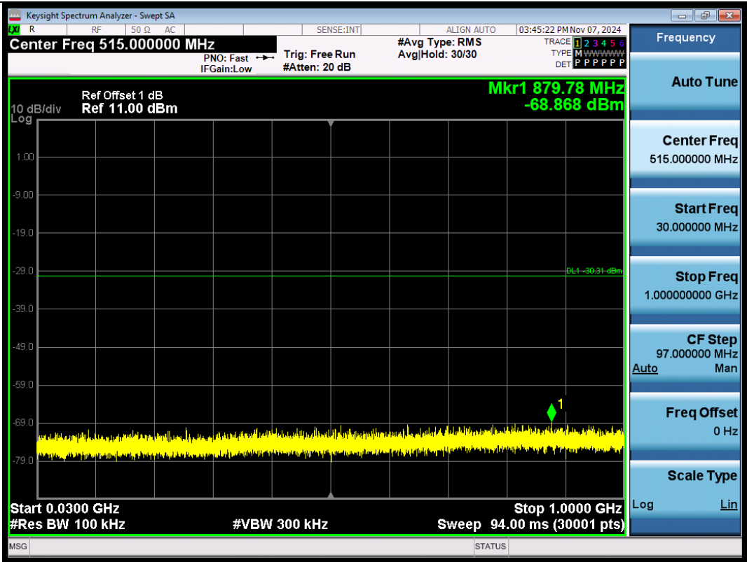
11AX20-2462-30~1000-PASS
