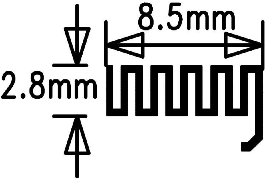
Antenna Photo & Length (mm)
