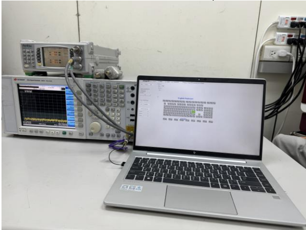
SRD2.4G_Conducted_Setup
