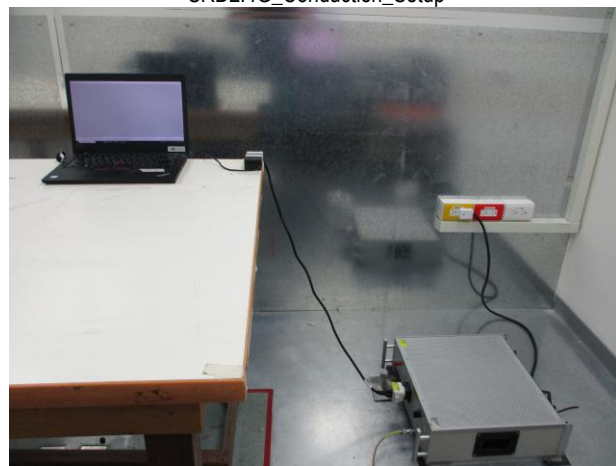
SRD2.4G_Conduction_Setup
