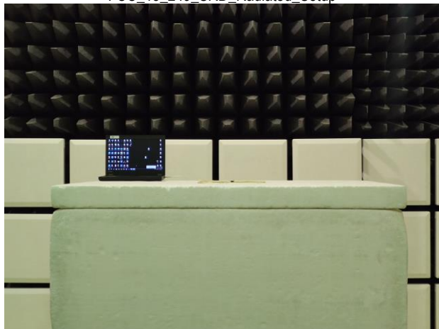
FCC 15_249_SRD_Radiated_Setup
