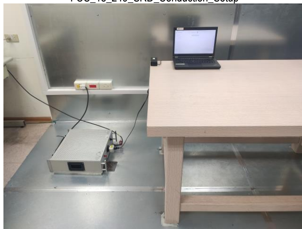
FCC 15_249_SRD_Conduction_Setup
