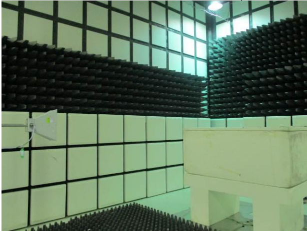
FCC_Part_15.247_SRD_Radiated_Setup
