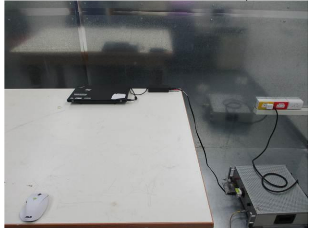
FCC_Part_15.247_SRD_Conduction_Setup
