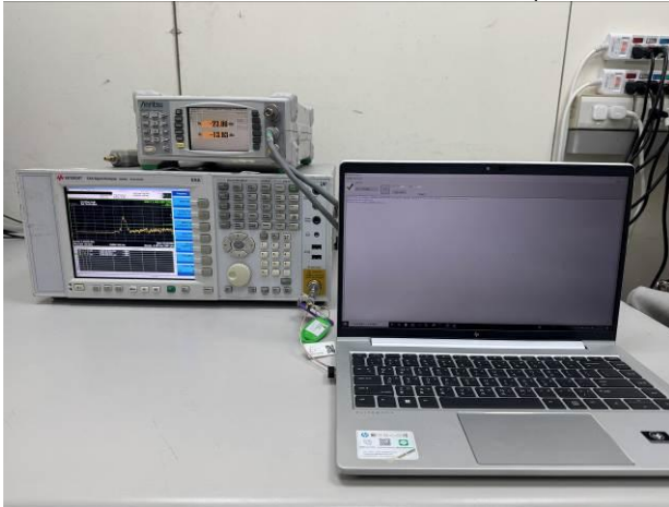
FCC Part 15.247 SRD Conducted Setup
