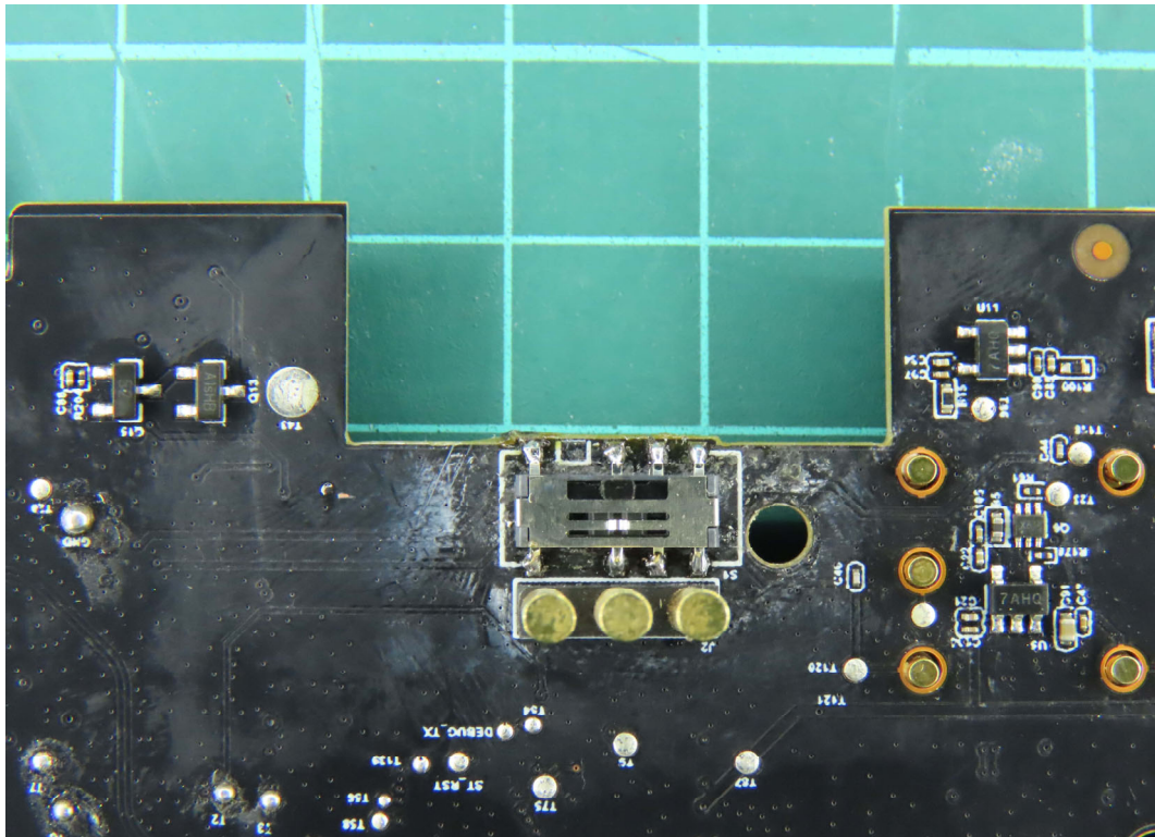
(55) EUT Photo
