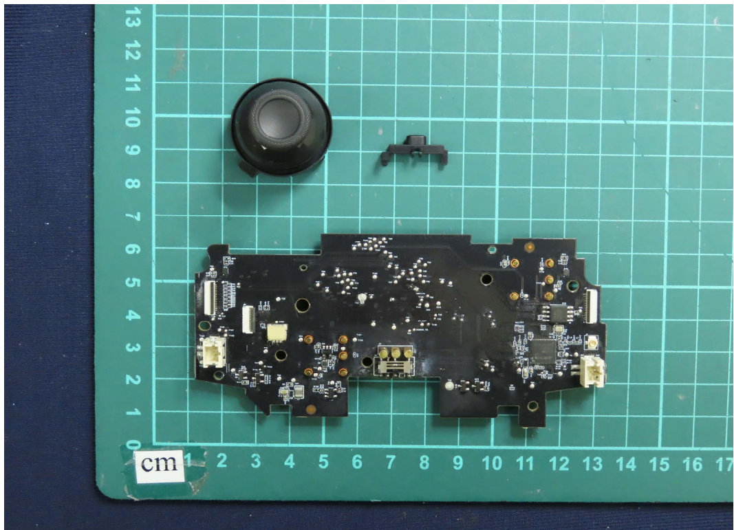
(51) EUT Photo
