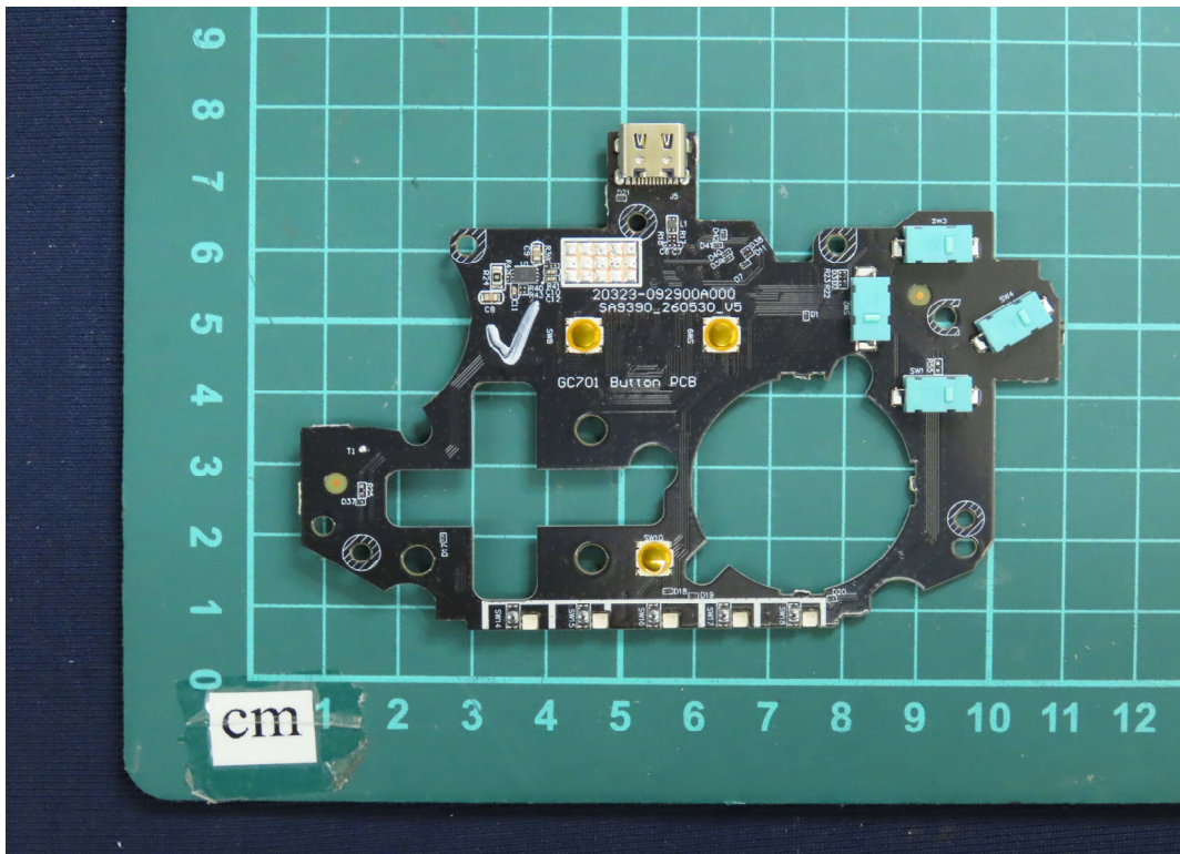
(63) EUT Photo (shipping version)
