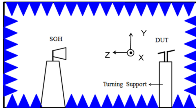
Chamber Coordinate System
