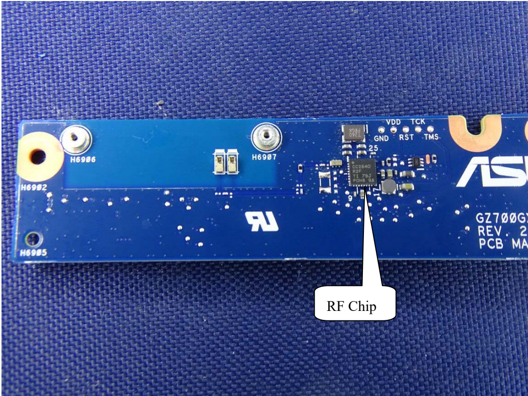
(32) EUT Photo
