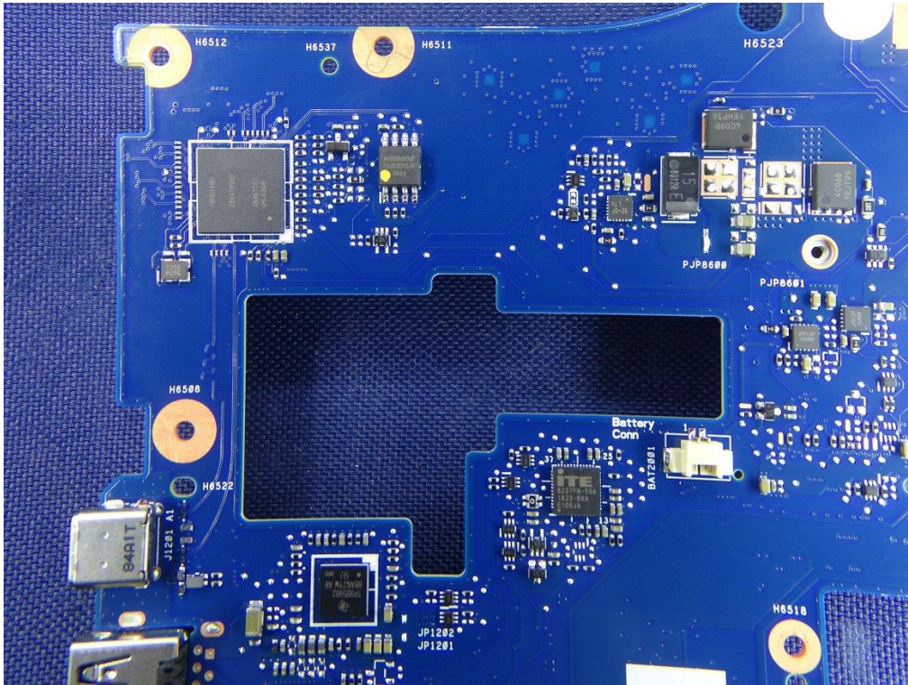
(55) EUT Photo
