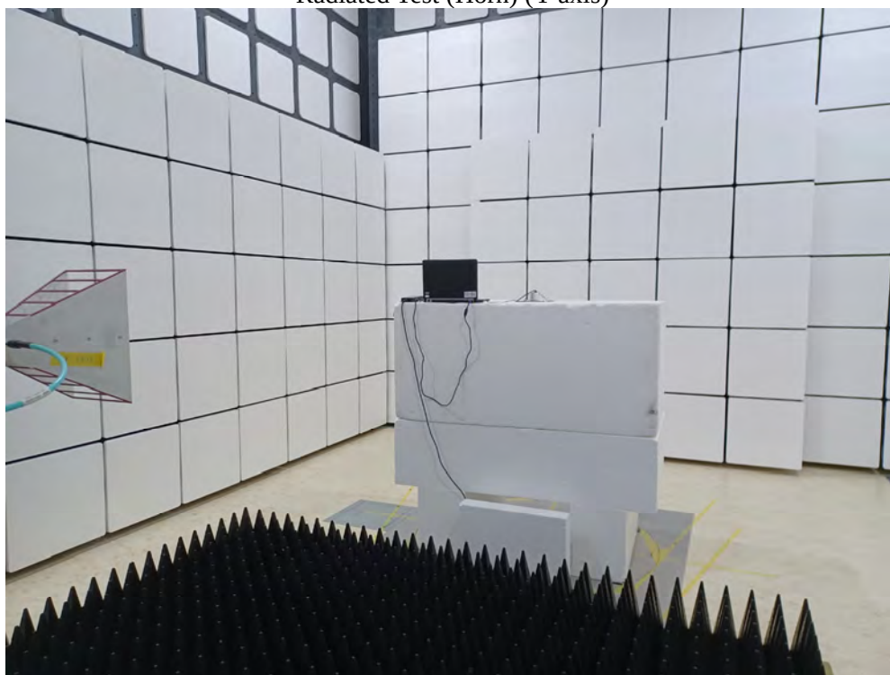
Radiated Test (Horn) (Y axis)
