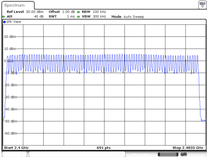
GFSK Mode
