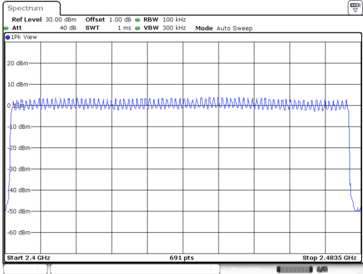
π/4-DQPSK Mode
