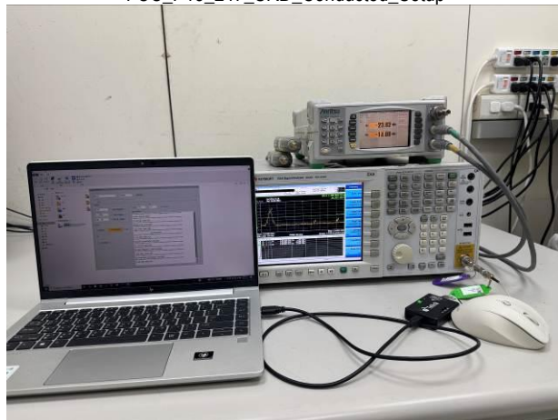
FCC_P15_247_SRD_Conducted_Setup
