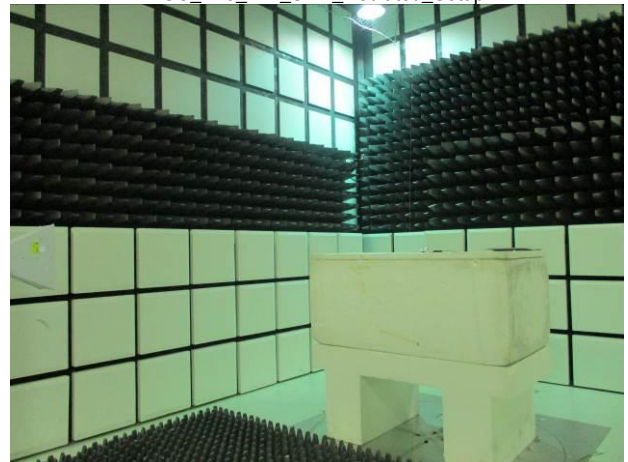
FCC_P15_247_SRD_Radiated_Setup
