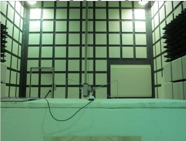
FCC_P15_247_BLE_Radiated_Setup
