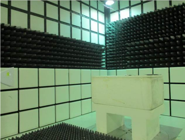
FCC_P15_247_BLE_Radiated_Setup
