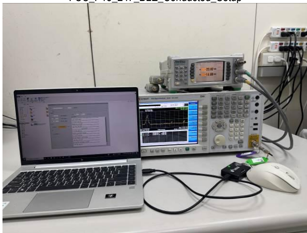
FCC_P15_247_BLE_Conducted_Setup
