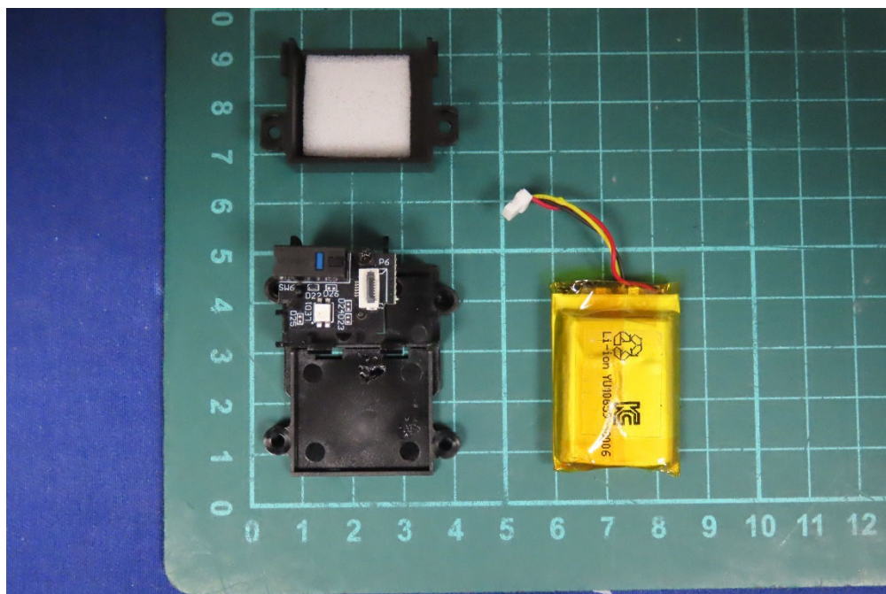
(7) EUT Photo
