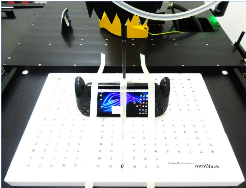
Setup for Power Density Testing (Bottom Side of DUT at 2 mm)
