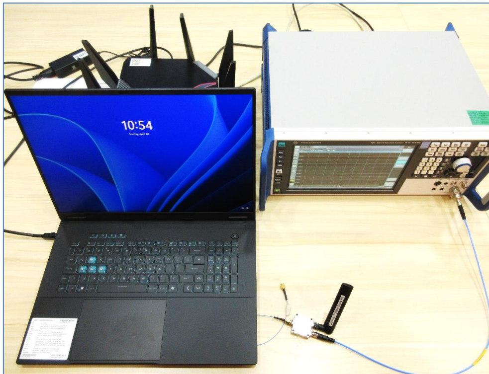
Setup for Conducted Power Testing (Test Scenario 1)
