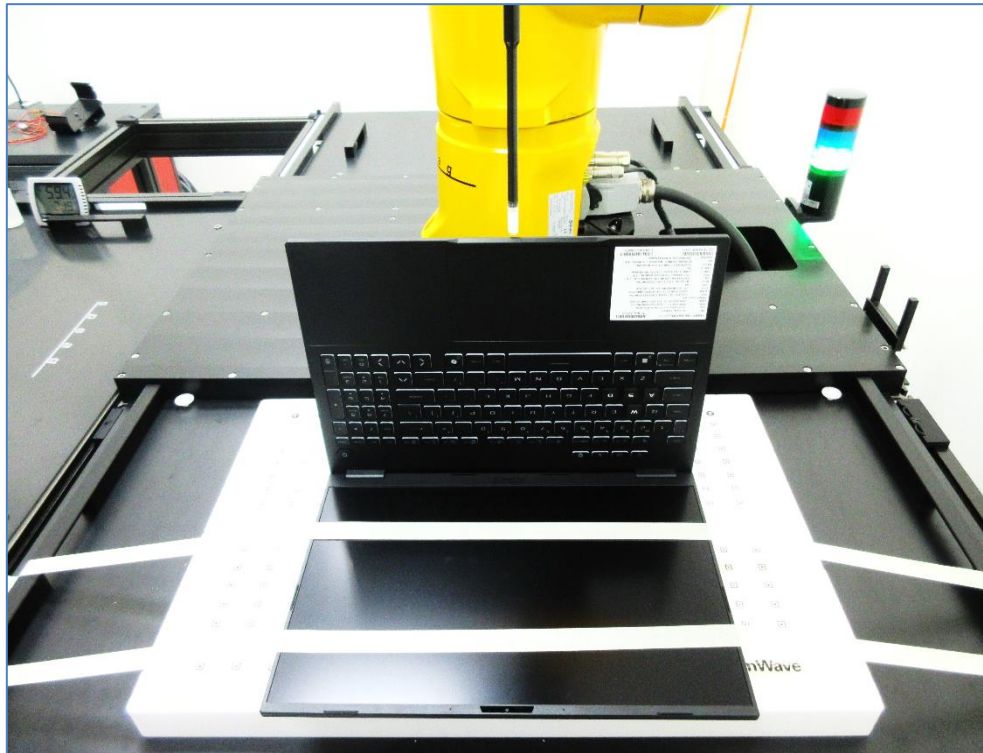
Setup for Power Density Testing (Front Edge of Laptop at 2 mm)
