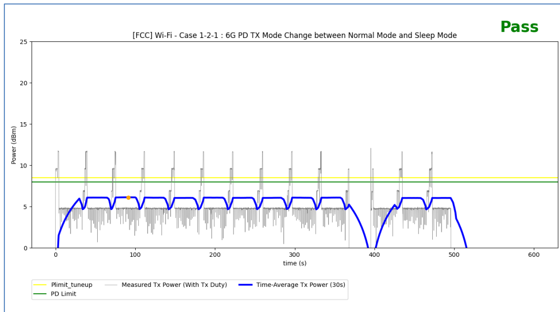
Figure 8-1: Time-Averaged Conducted TX Power Over Time for Wi-Fi Test Scenario 1
