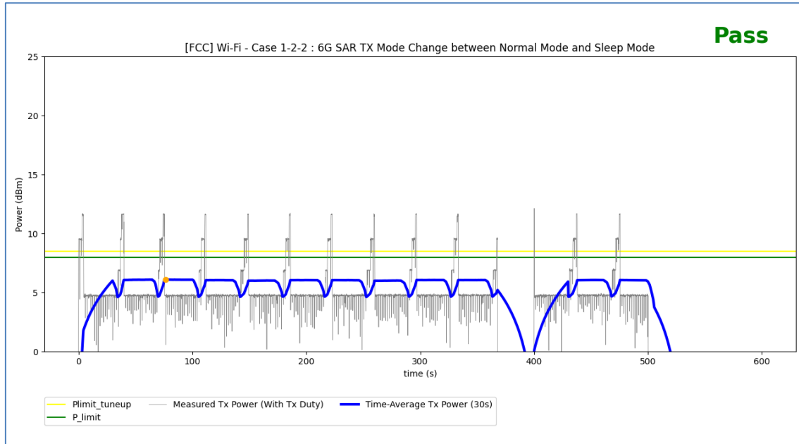
Figure 6-6: Time-Averaged Conducted TX Power Over Time for Wi-Fi Test Scenario 1-2
