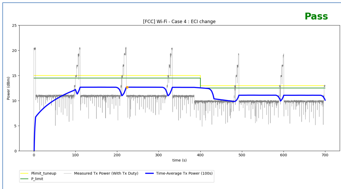
Figure 6-11: Time-Averaged Conducted TX Power Over Time for Wi-Fi Test Scenario 4
