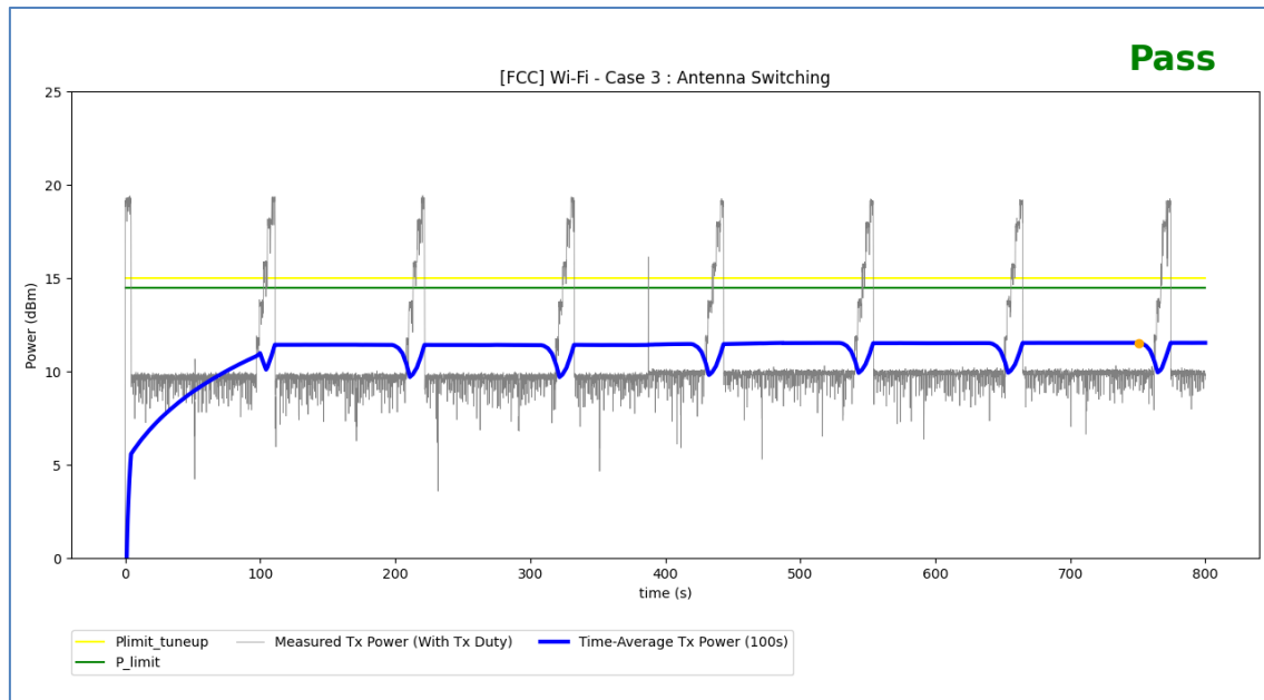
Figure 6-9: Time-Averaged Conducted TX Power Over Time for Wi-Fi Test Scenario 3
