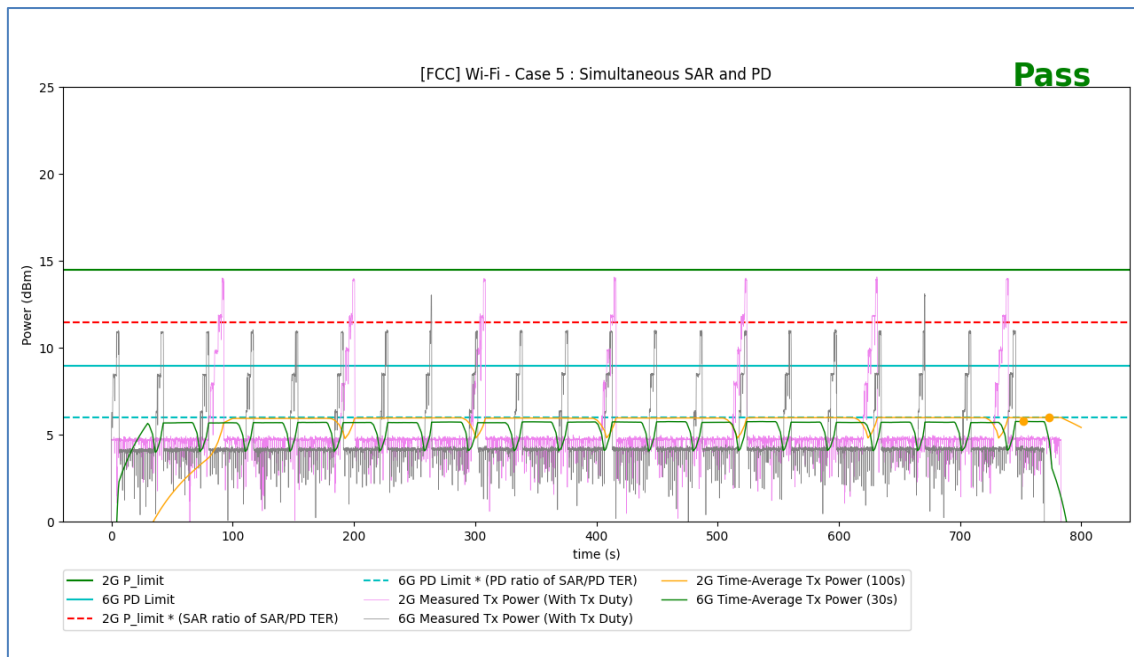
Figure 6-13: Time-Averaged Conducted TX Power Over Time for Wi-Fi Test Scenario 5
