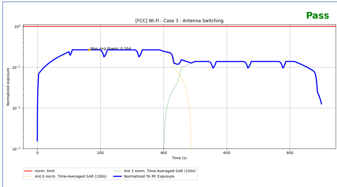
Figure 6-10: Normalized Time-Averaged SAR Over Time for Wi-Fi Test Scenario 3
