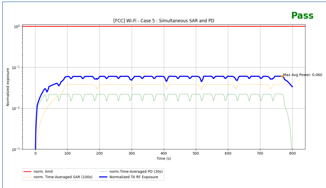
Figure 6-14: Total Normalized Time-Averaged RF exposure Over Time for Wi-Fi Test Scenario 5
