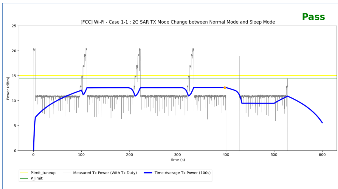
Figure 6-5: Time-Averaged Conducted TX Power Over Time for Wi-Fi Test Scenario 1-1
