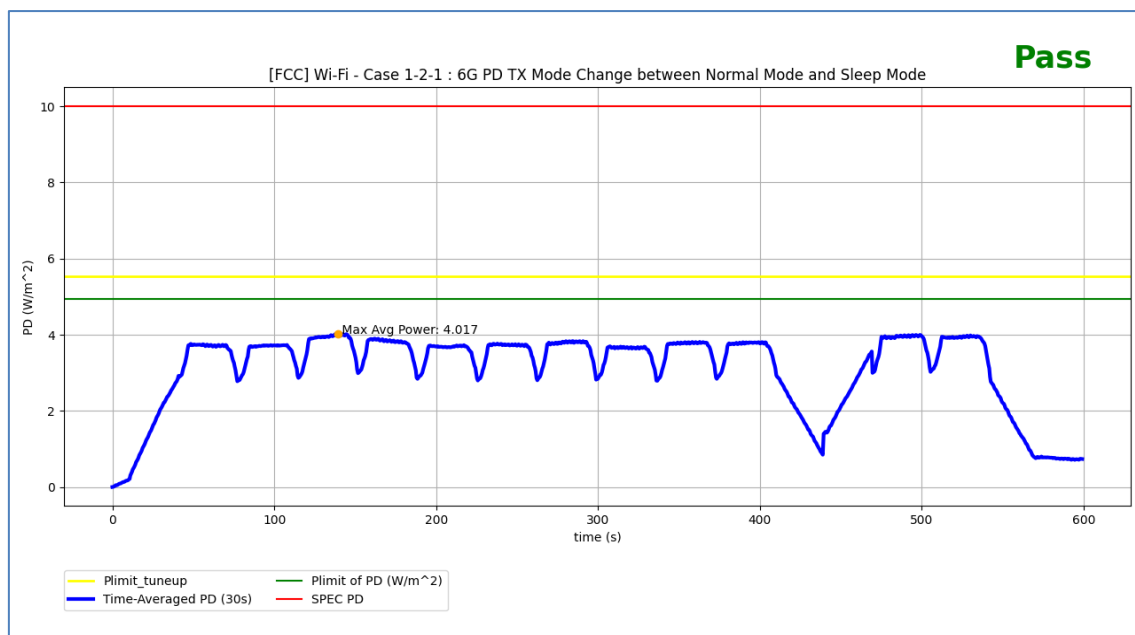
Figure 9-2: Time-Averaged PD Measurement Result for Wi-Fi Test Scenario 1
