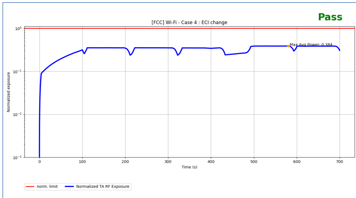
Figure 6-12: Normalized Time-Averaged SAR Over Time for Wi-Fi Test Scenario 4
