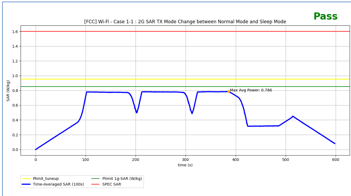
Figure 7-2: Time-Averaged SAR Measurement Result for Wi-Fi Test Scenario 1-1
