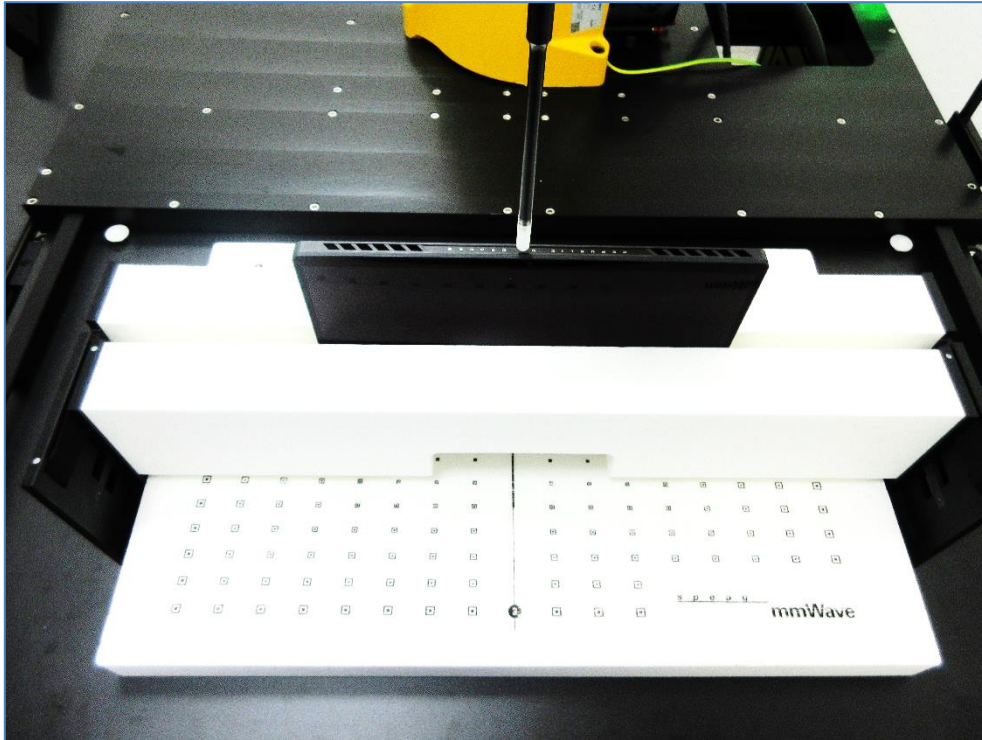
Setup for Power Density Testing (Tablet - Top Side at 2 mm)
