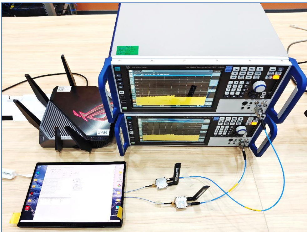
Setup for Conducted Power Testing (Test Scenario 2 and 5)
