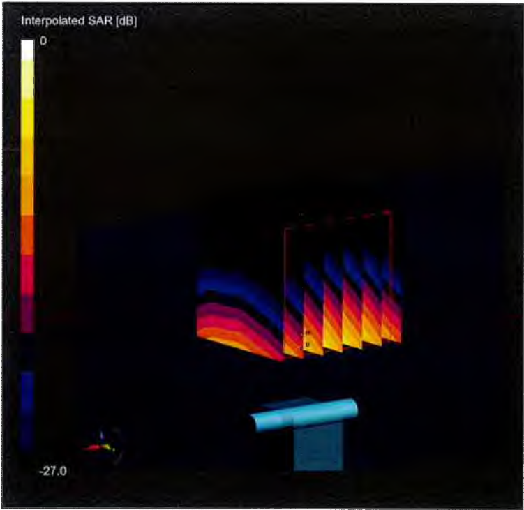
0 dB = 32.1 W/Kg
