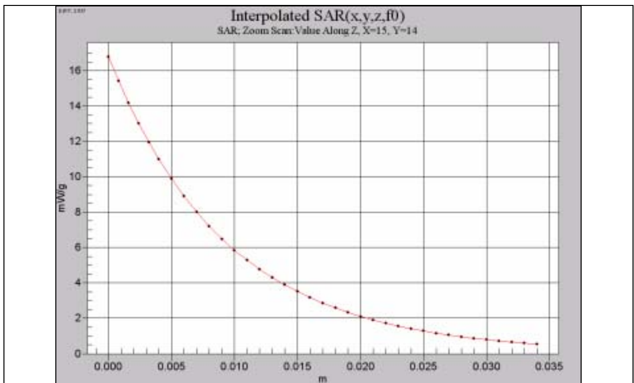
Body-Tissue-Simulating-Liquid 1900MHz
