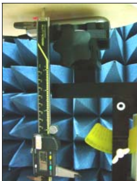
Figure 18. Body SAR Test Setup (Flat Section)
