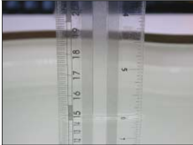
Figure 8. Head-Tissue-Simulating-Liquid 1900MHz
