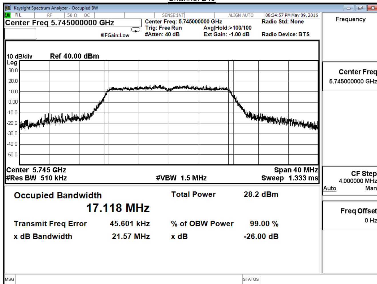
Channel 149
