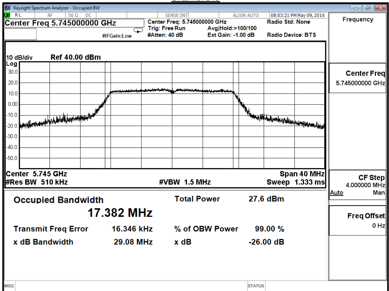
Channel 149
