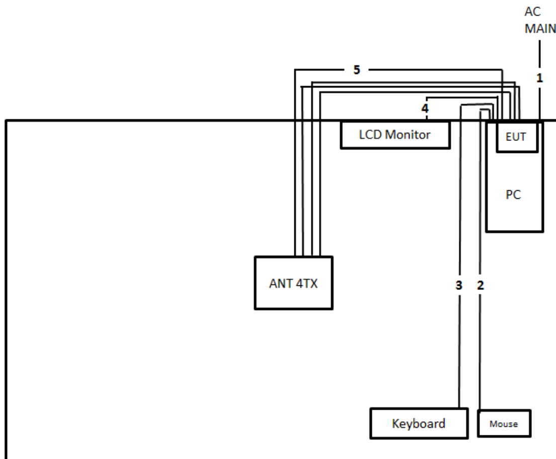
Test Setup Diagram - Radiated Test < 1GHz Non-Beamforming Mode (above 1GHz)
