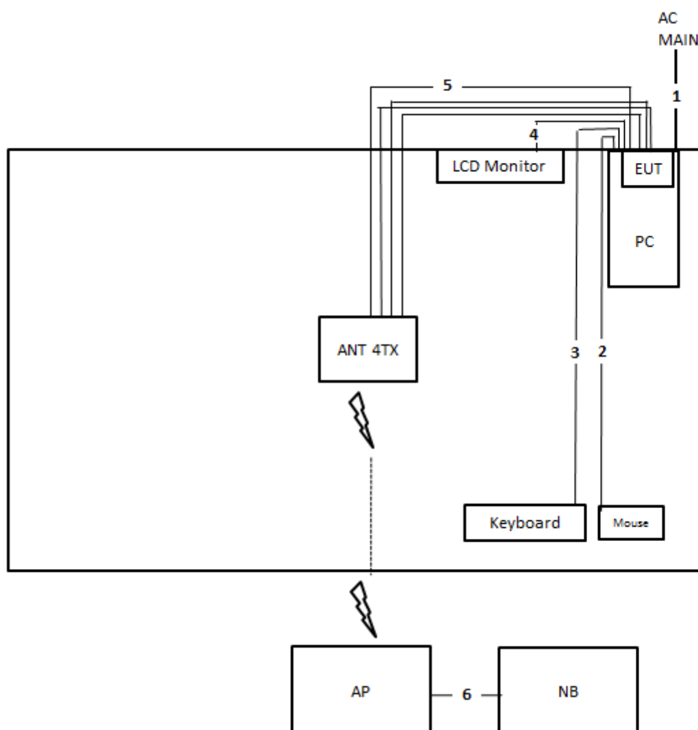
Test Setup Diagram - Radiated Test > 1GHz and Beamforming Mode
