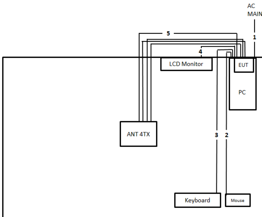
Test Setup Diagram - Radiated Test > 1GHz and Non-Beamforming Mode
