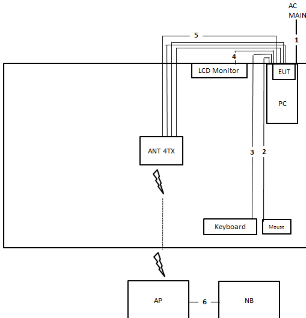
Test Setup Diagram - Radiated Test > 1GHz Beamforming Mode
