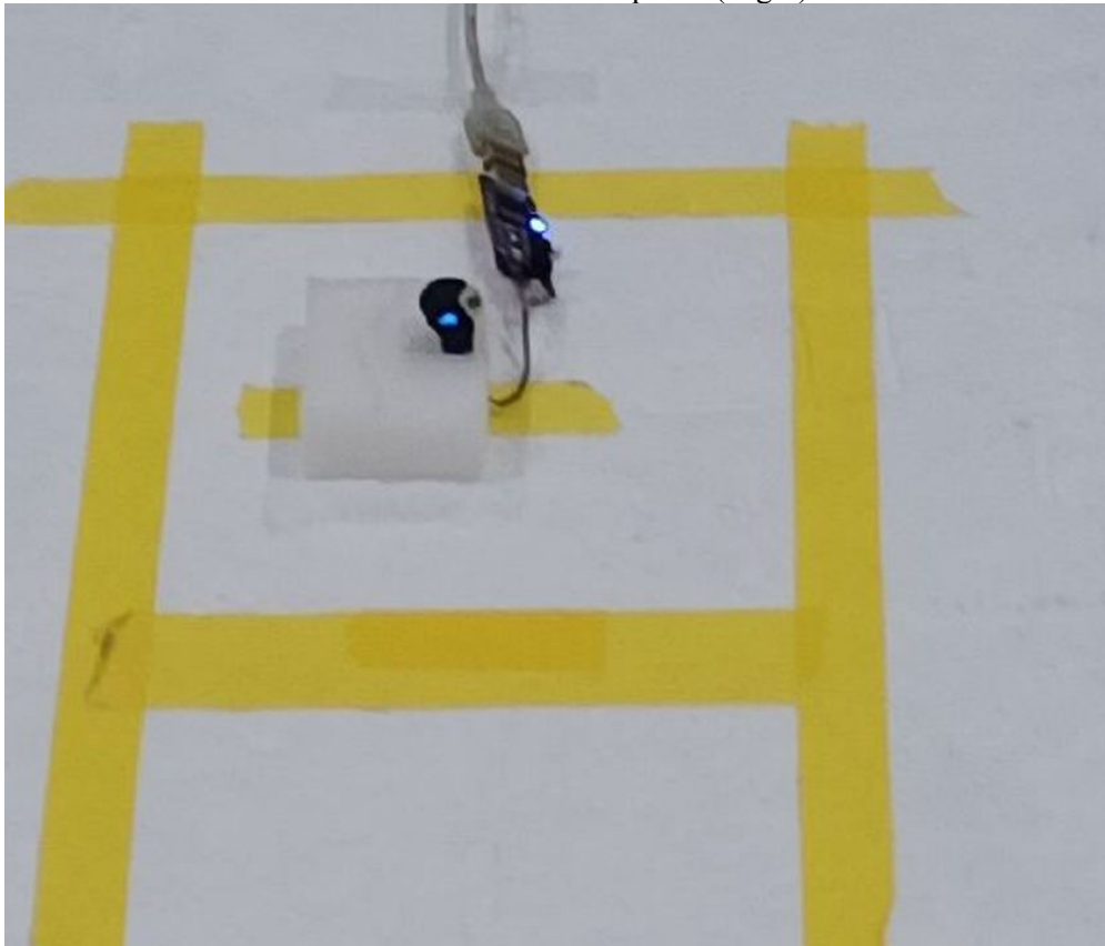
Radiated Test - zoom-in photo (Charger)
