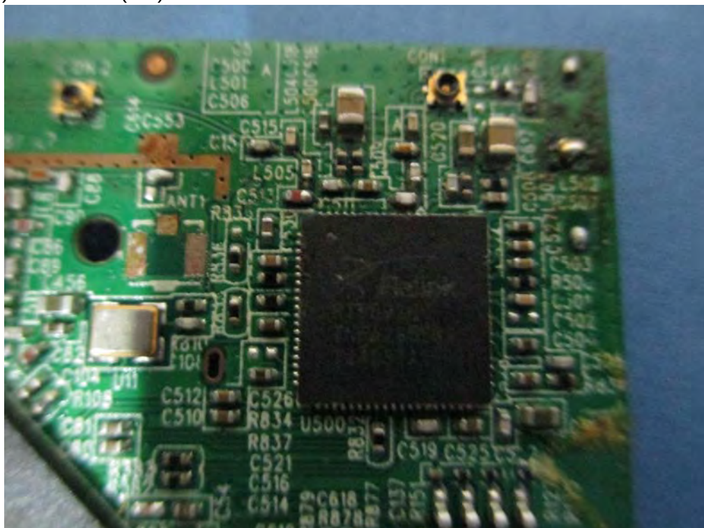
(38) EUT Photo (MB)
