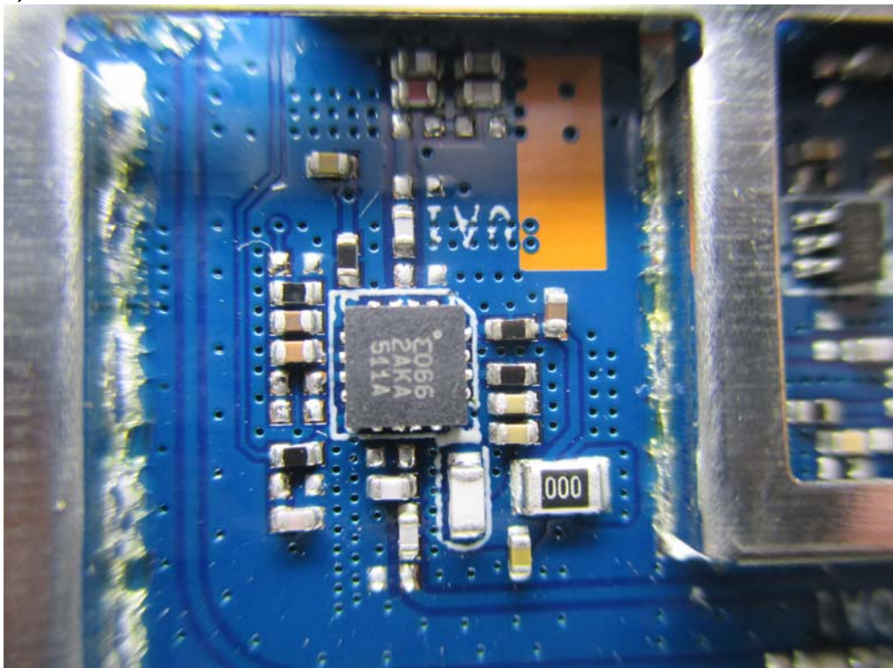
(26) EUT Photo
