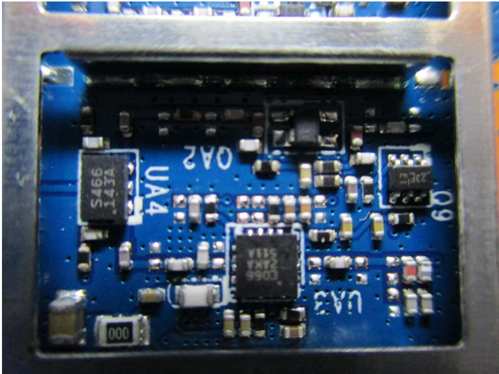
(23) EUT Photo
