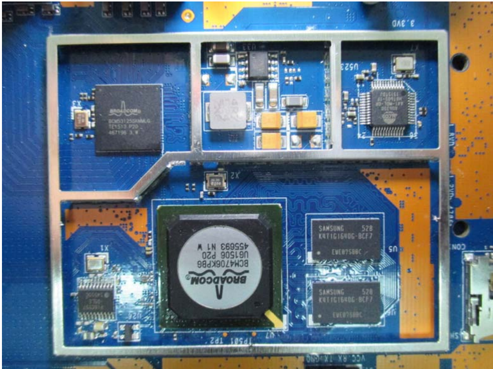
(27) EUT Photo
