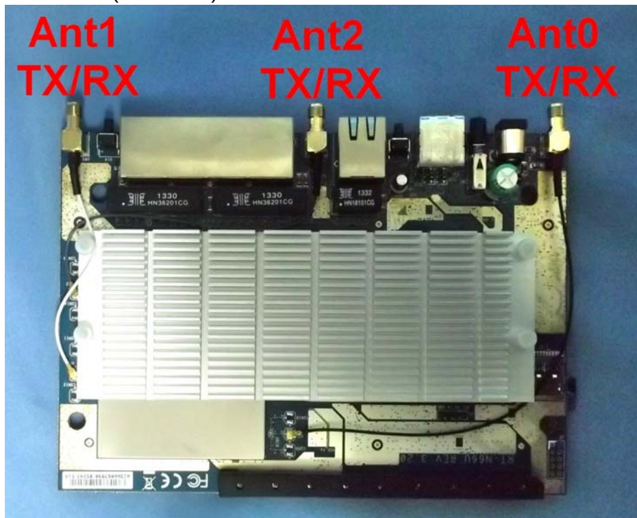
(34) EUT Photo (3TX / 3RX)
