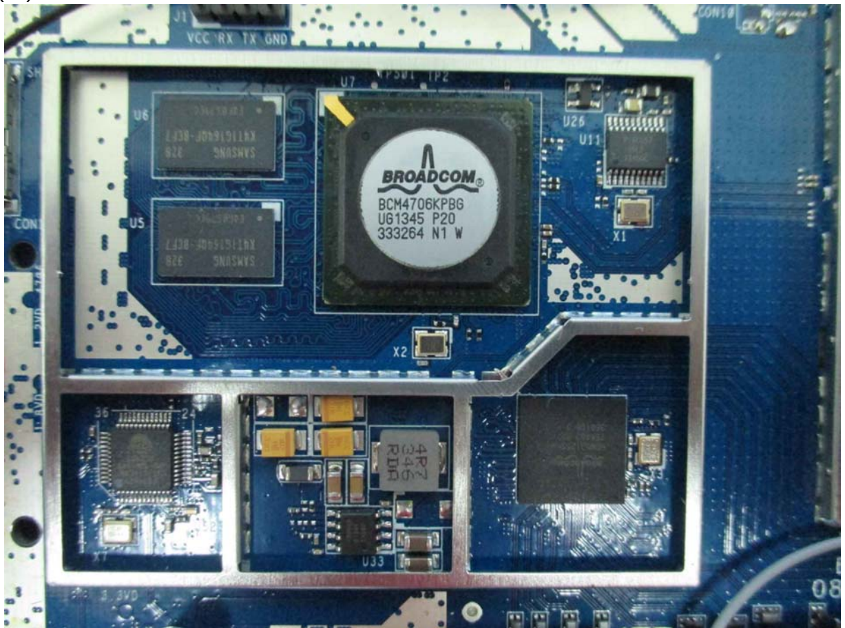
(28) EUT Photo
