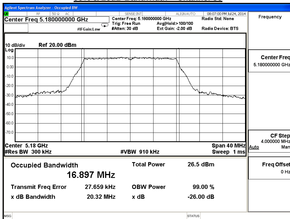
99% & 26dB Bandwidth – Channel 36
