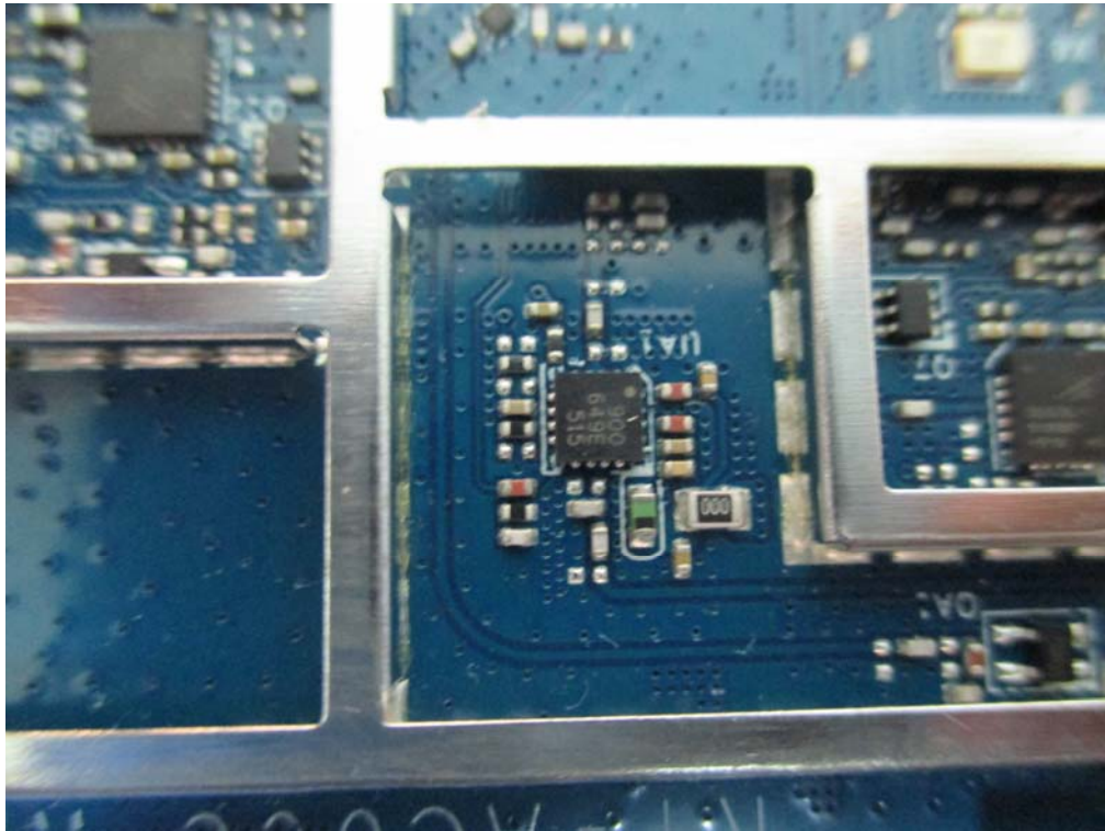
(21) EUT Photo (PA)
