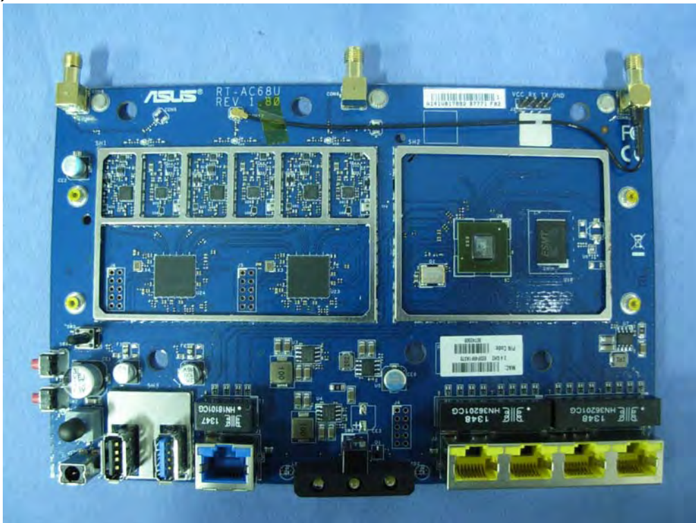
(26) EUT Photo
