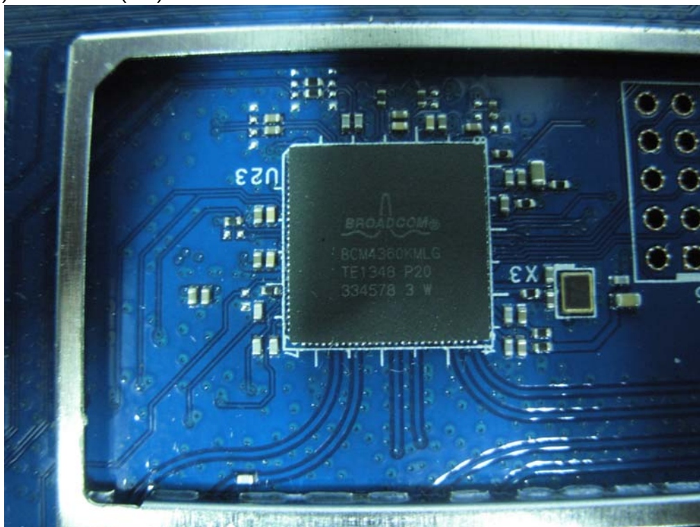
(46) EUT Photo (MB)
