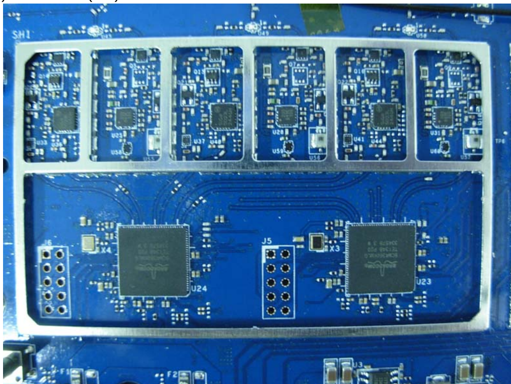
(44) EUT Photo (MB)
