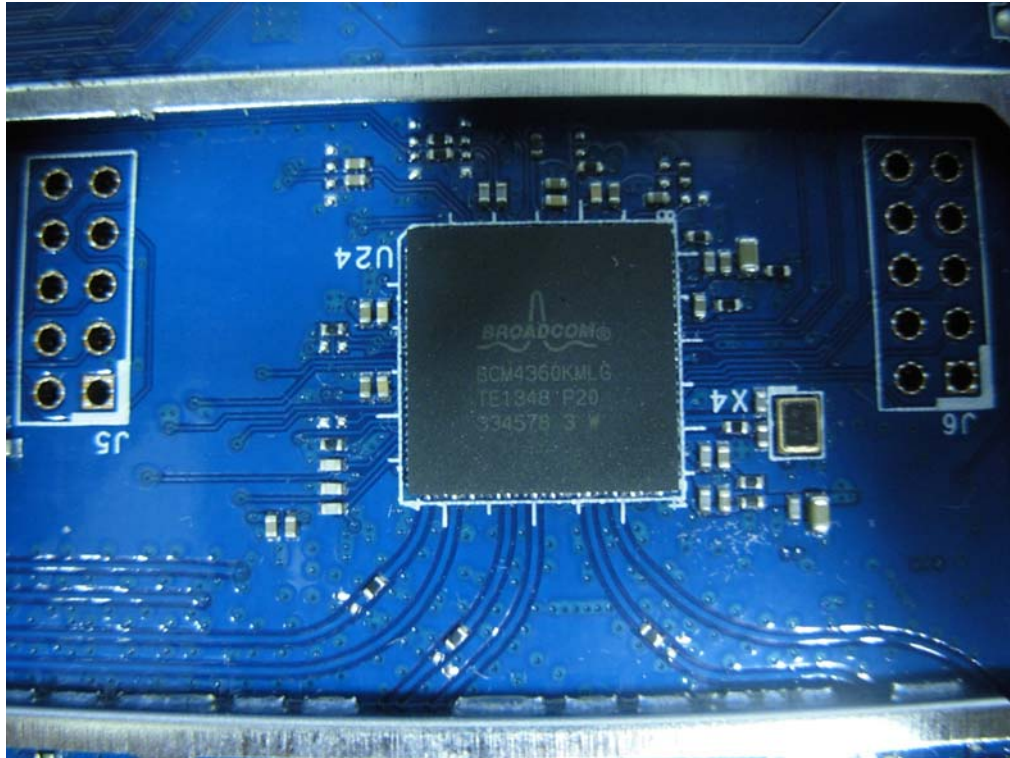
(47) EUT Photo (MB)
