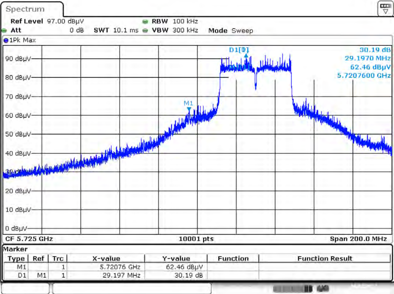
RF antenna conducted test - Channel 151
