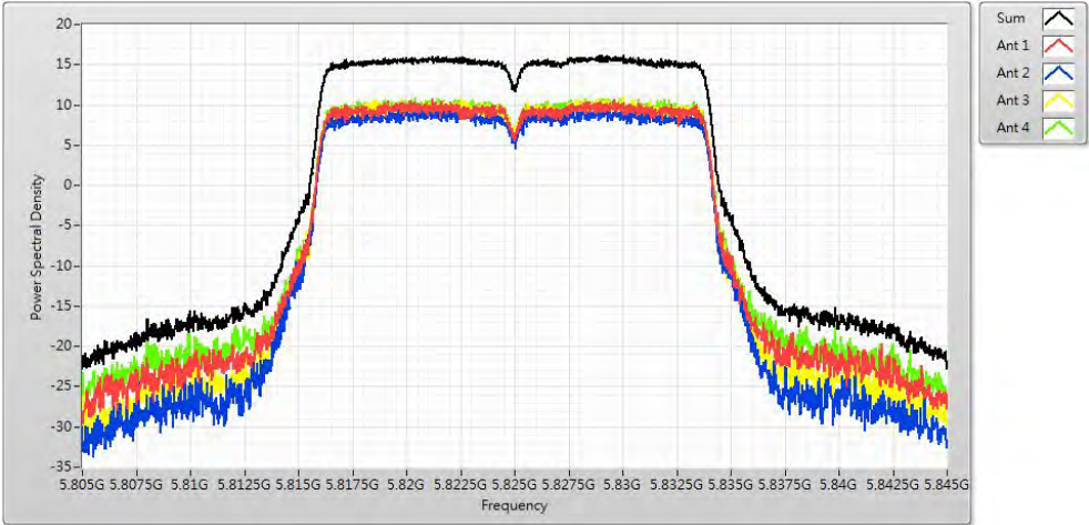
Channel 165
