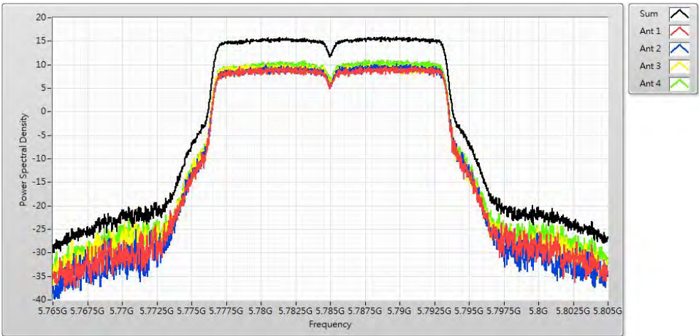
Channel 157
