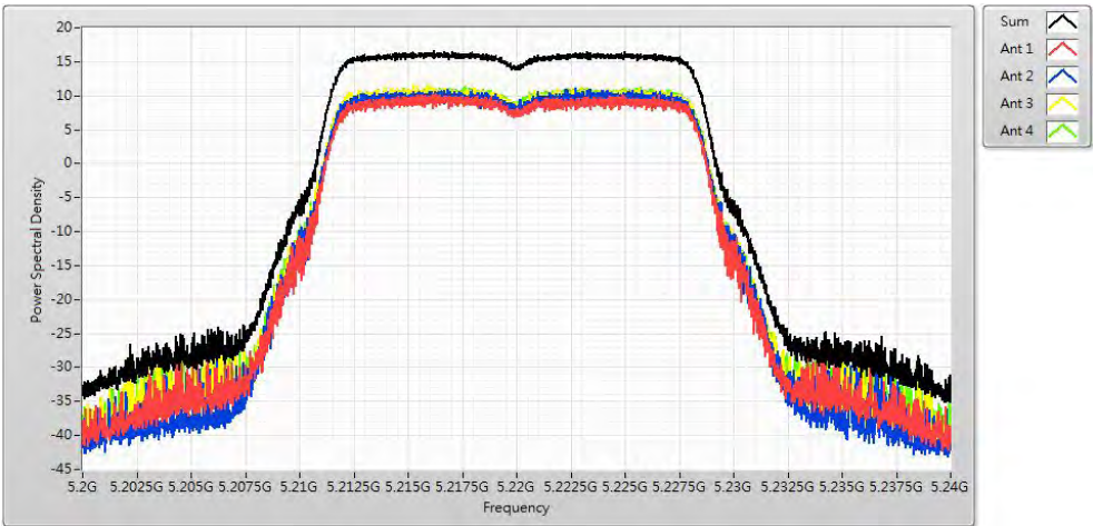
Channel 44
