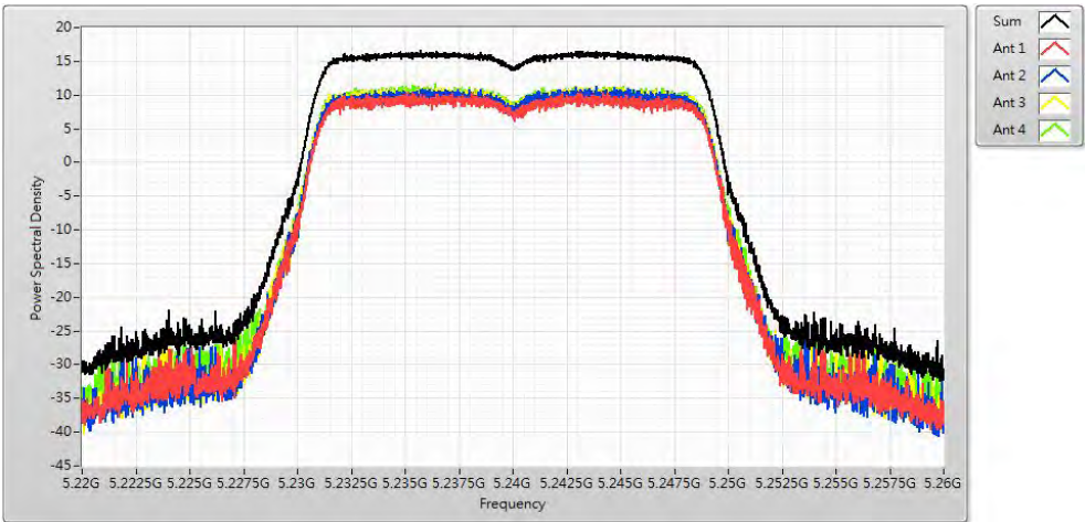
Channel 48
