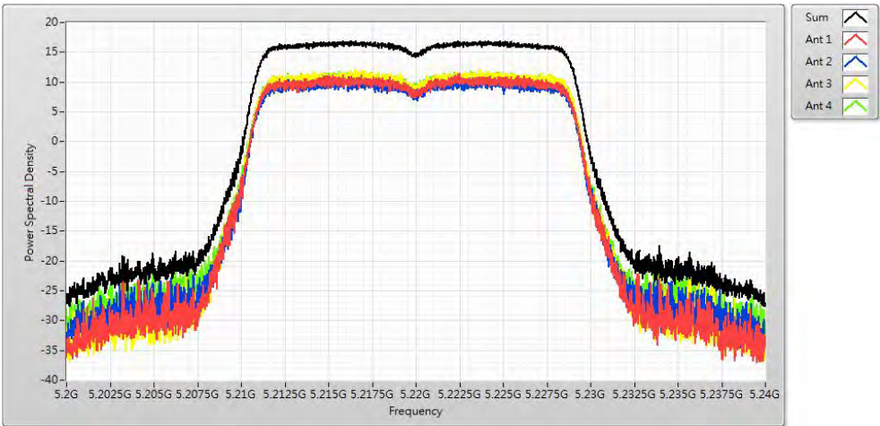
Channel 44
