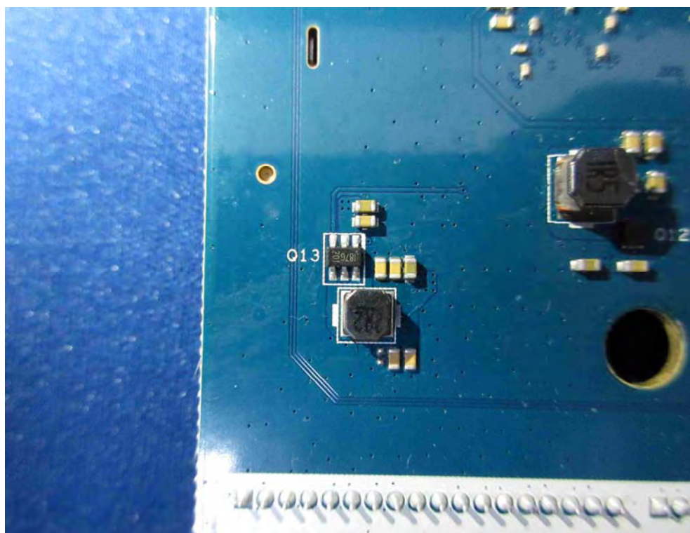
(7) EUT Photo
