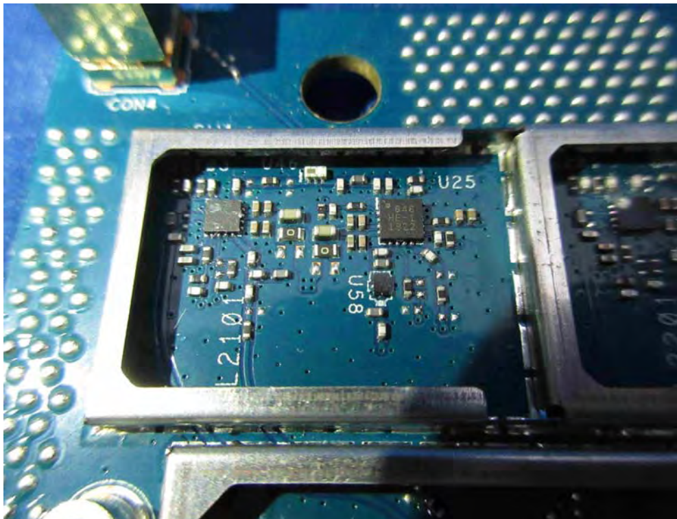
(34) EUT Photo
