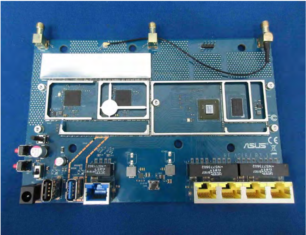
(22) EUT Photo
