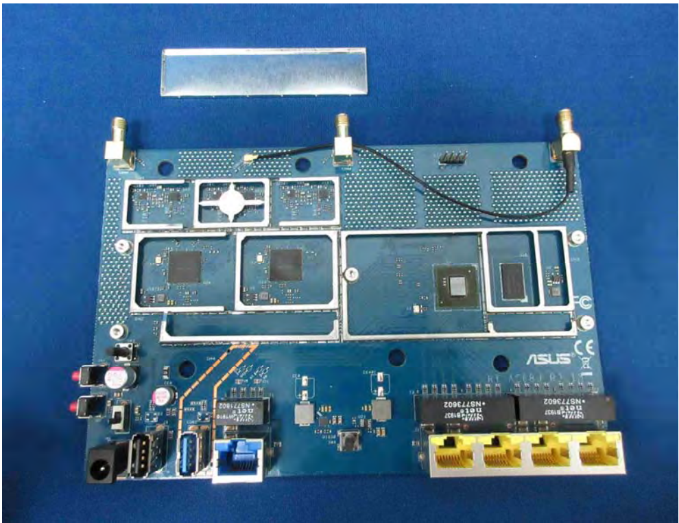
(32) EUT Photo
