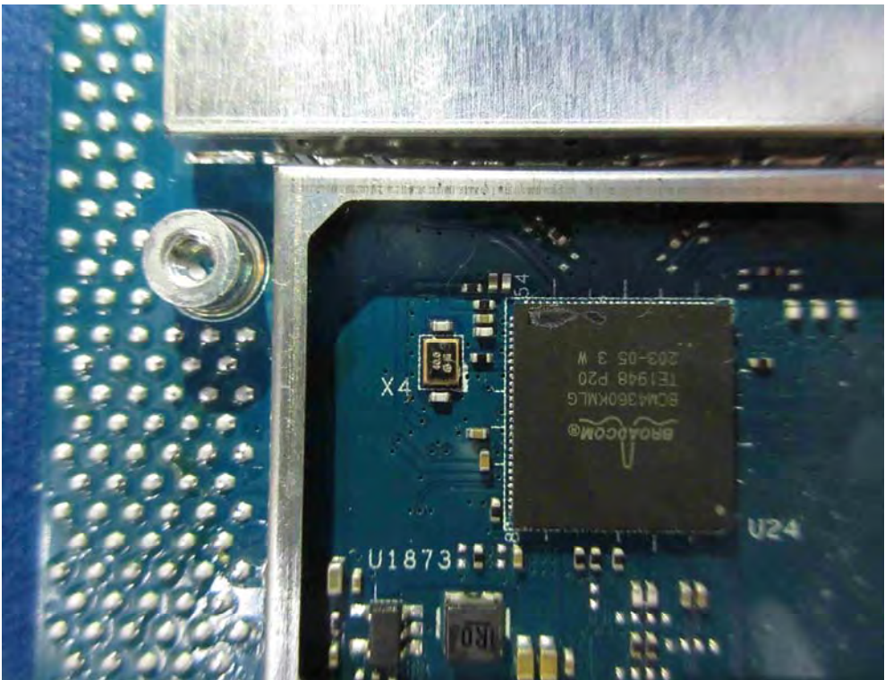
(28) EUT Photo
