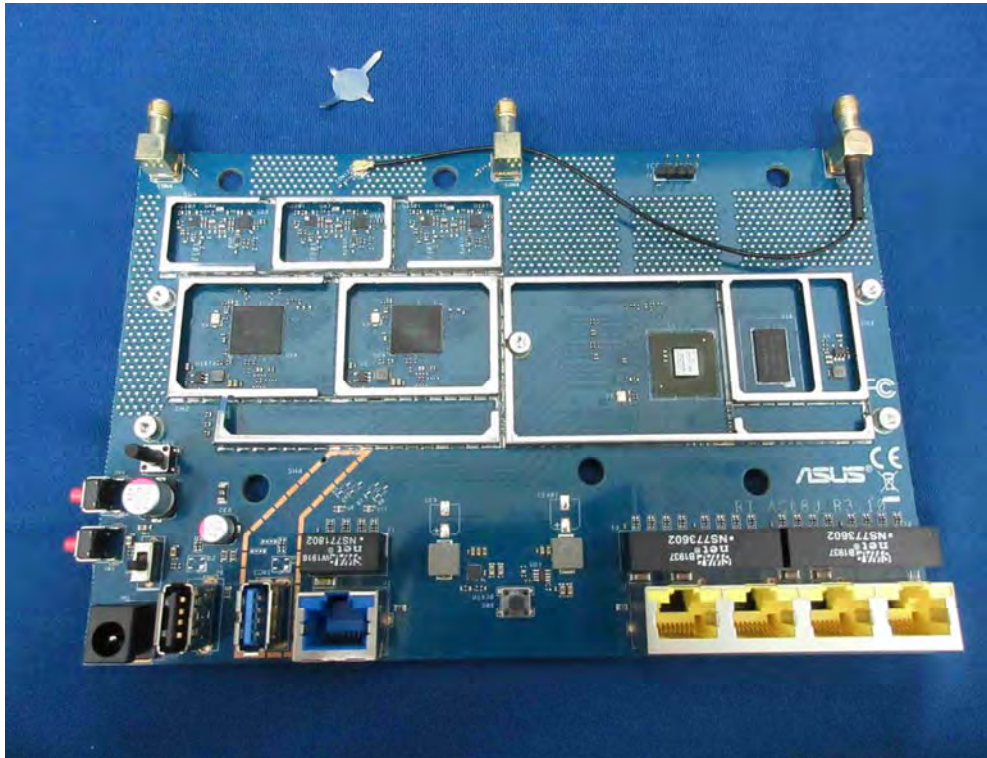
(34) EUT Photo
