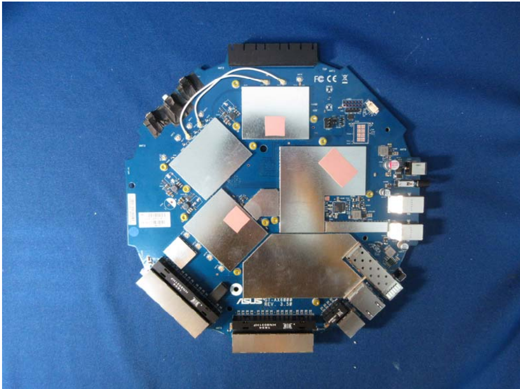
(6) EUT Photo(M/N: GT-AX6000-Transformer 2)
