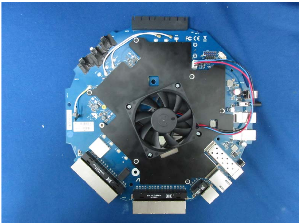
(9) EUT Photo (M/N: GT-AX6000-fan_Transformer 2)
