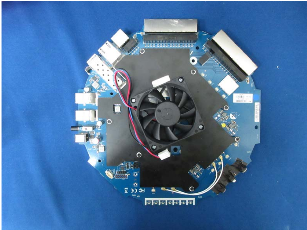
(8) EUT Photo (M/N: GT-AX6000-fan_Transformer 1)
