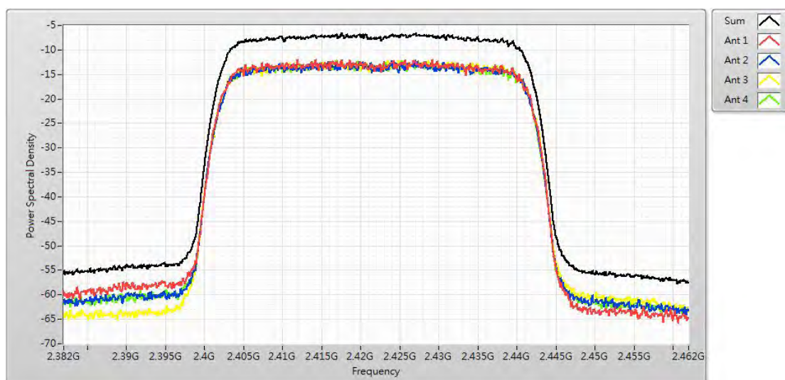
Channel 3 (2422MHz)
